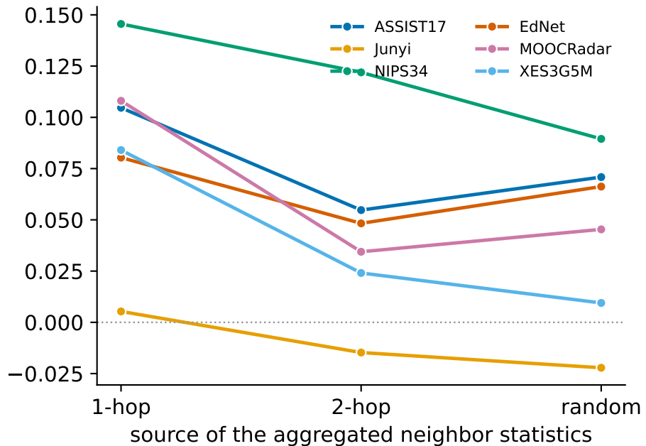
(b) neighbor information by graph distance
