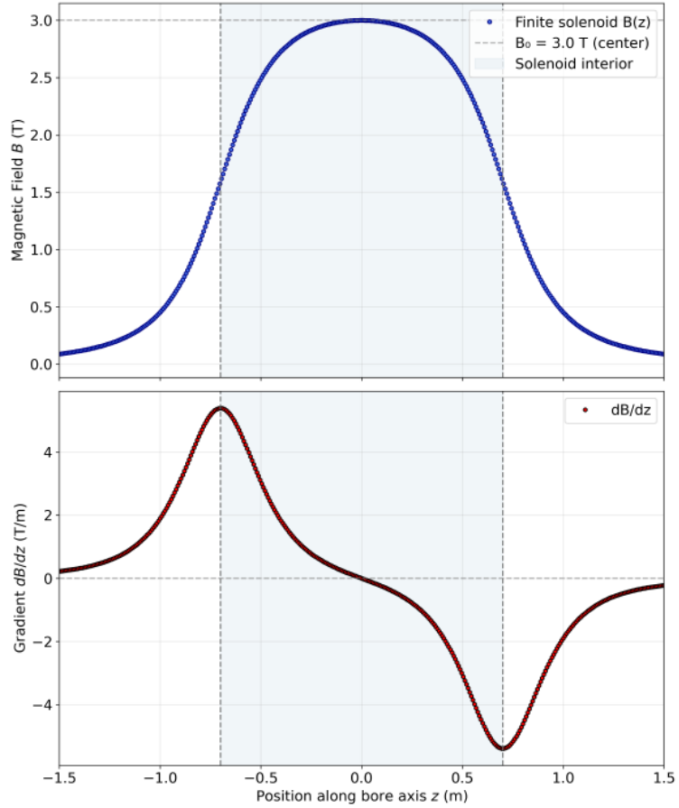
Figure 2.2: Axial magnetic flux density B_z and spatial gradient for an idealized 3 T MRI solenoid ( L = 1.4 m, R = 0.3 m). Top: The magnetic field peaks at 3T at the isocenter ( z = 0 m) and decreases symmetrically toward both ends. Grey dotted lines indicate the solenoid edges (bore entrances). Bottom: The spatial gradient dB_z/dz reaches its maximum magnitude at the bore entrances ( z = \pm 0.704 m).
