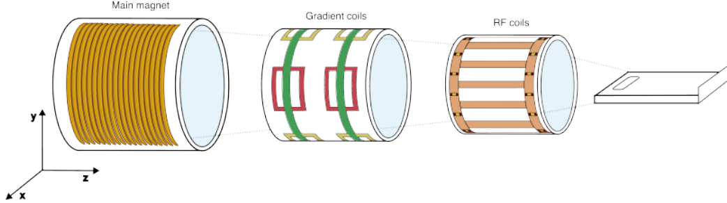
Figure 2.1: Exploded view of an MRI scanner: the main magnet, gradient coils, RF system and patient couch.
