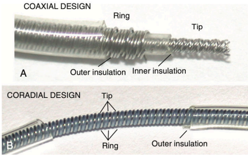
Figure 2.6: Body design variations in pacing bipolar leads. Coaxial designs use two nested coil conductors with separate insulation layers, whereas co-radial designs incorporate parallel, intertwined conductors within a shared lumen. Reprinted from Clinical Cardiac Pacing, Defibrillation, and Resynchronization Therapy , Haqqani et al., p. 133, Copyright (2011), with permission from Elsevier [2].
