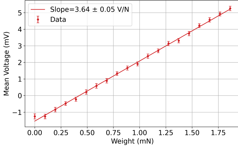
Figure 4.11: Calibration of aluminum sensor for masses ranging from 0 to 200 mg.
