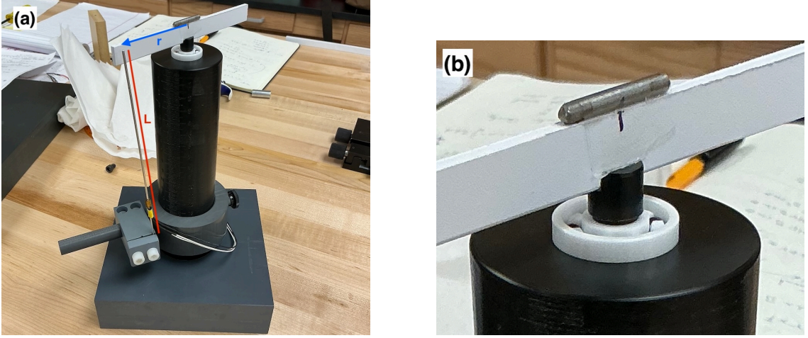
Figure 3.14: Non-magnetic torque fixture designed for horizontal test object orientation. (a) The torque fixture pole provides rigid support. The key adjustable parameters for maximizing measured torque are the sensor's tip position L (red) and the distance from center to sensor along the transfer arm r (blue). (b) Close up of the transfer arm on top of fixture (from bottom to top): magnetically susceptible test object, Kydex ™ transfer arm, plastic alignment notch, and ceramic bearing for low-friction rotation.
