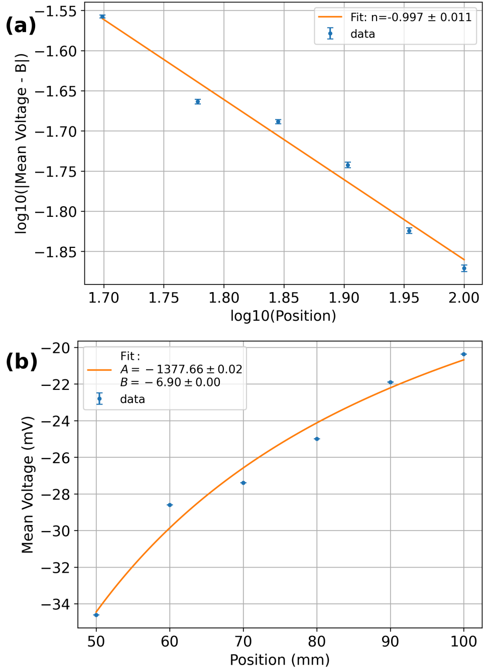
Figure E.4: Demonstration of the expected inverse-distance dependence of the force (and thus torque) with respect to the distance r from the rotation axis. Both analyses confirm the 1/r dependence characteristic of the torque measurement via counter-force method. (a) Log-log plot of effective measured voltage (proportional to force) versus position r , showing a power-law fit with exponent n = -0.997 \pm 0.011 , very close to the theoretically expected value of -1 . (b) Direct fit of the form F(r) = A/r + B , yielding A = -1.378 \pm 0.015 (very close to -1 in normalized units) and a negligible offset B = -0.0069 \pm 0.0002 .
