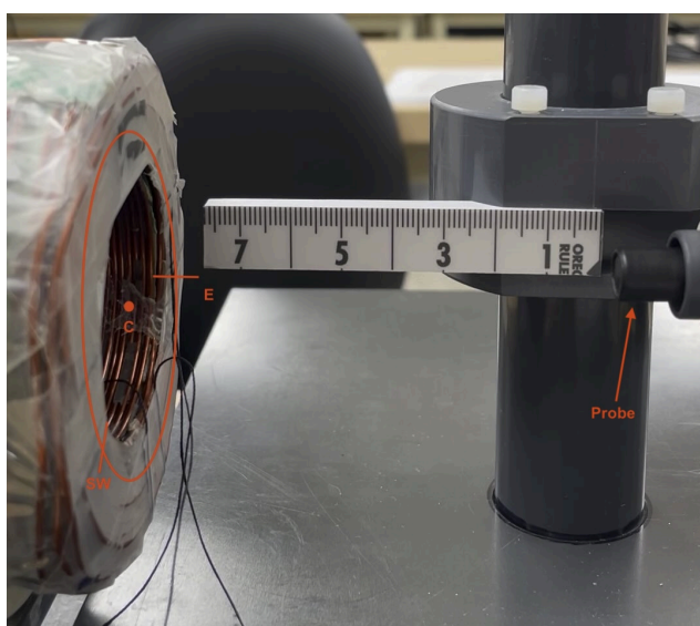
Figure 3.3: Probe mapping magnetic field generated from solenoid.
