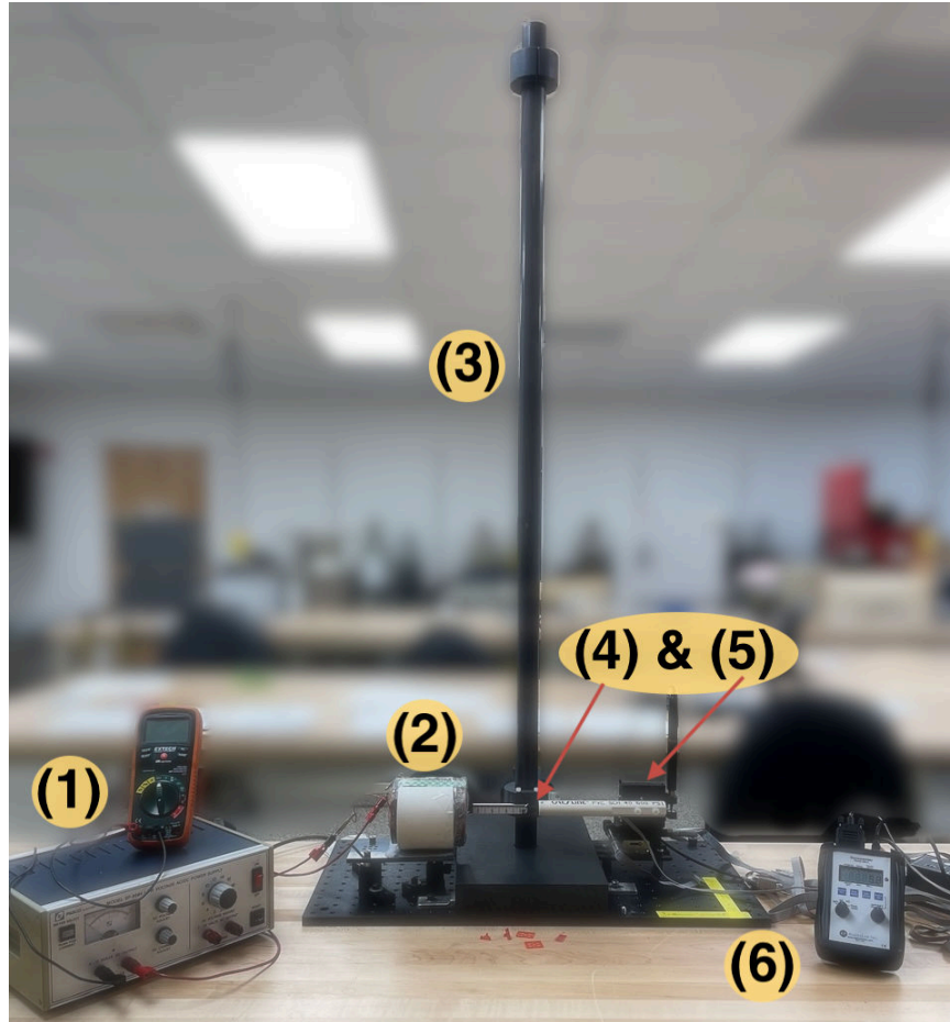
Figure 3.11: Laboratory setup for MRI translational force assessment. (1) Magnetic field generation instruments (left), (2) solenoid, (3) fixture with pole (center), (4) gaussmeter probe, (5) translation stage, and (6) gaussmeter read panel (right).
