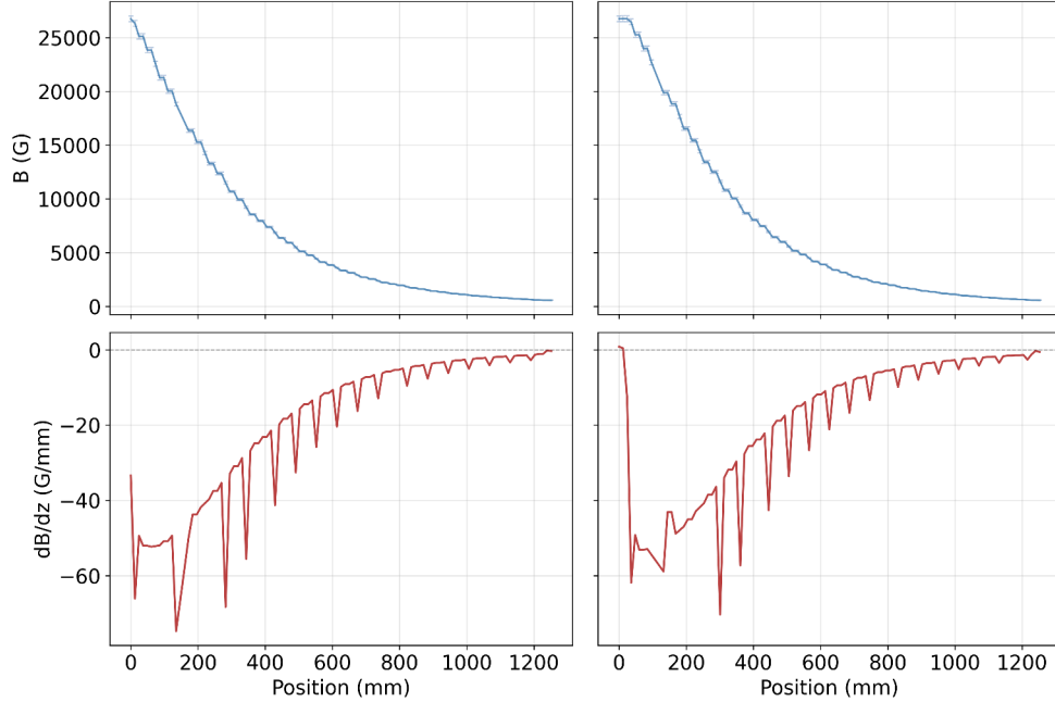
Figure 3.6: Magnetic field(top row) and corresponding gradient (bottom row) along the measurement path after converting time to position but prior to separating repeated measurements.
