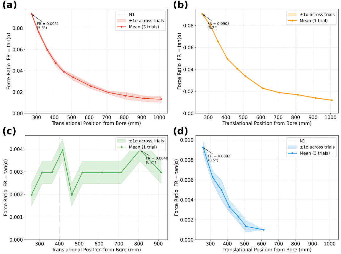
Figure 4.7: Magnetically Induced Displacement Force – ASTM F2052-15[7]. Force Ratio FR = \tan(\alpha) vs. z-axis Position. (a) Unipolar Epicardial Lead. (b) 316 Stainless Steel straight wire. (c) Titanium straight wire. (d) Titanium coiled wire.
