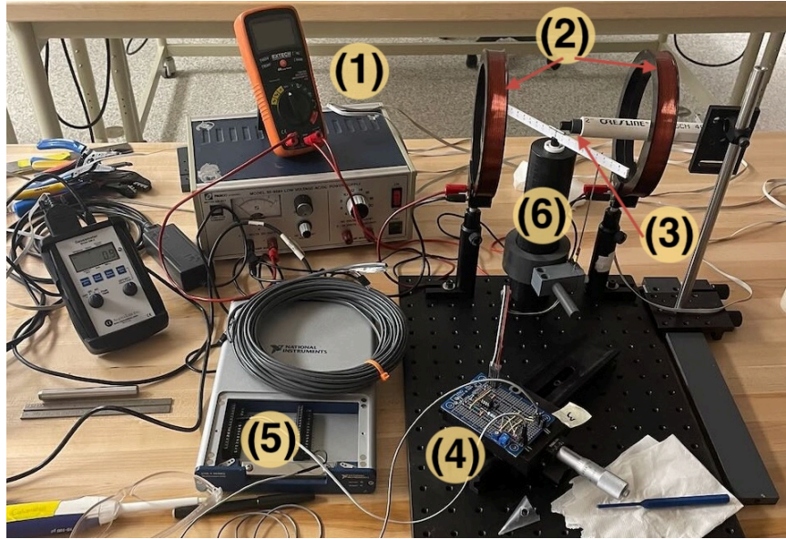
Figure 3.21: Experimental setup for torque measurements. Includes magnetic field generation and measurement devices, (1) through (3). (4) is the sensor circuit, (5) is the DAQ system connected to a laptop. (6) is the main device where the test object sits.
