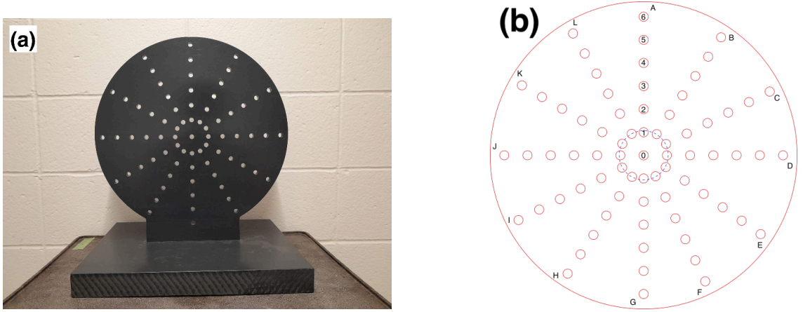
Figure 3.2: PVC-based magnetic field mapping platform and coordinated circular grid layout labeled from A to L angular and from 0 to 6 radial. This platform was used for spatial B_0 and \nabla B_0 measurement, based on design from Ferreira, et al. (2017) [35, 31].
