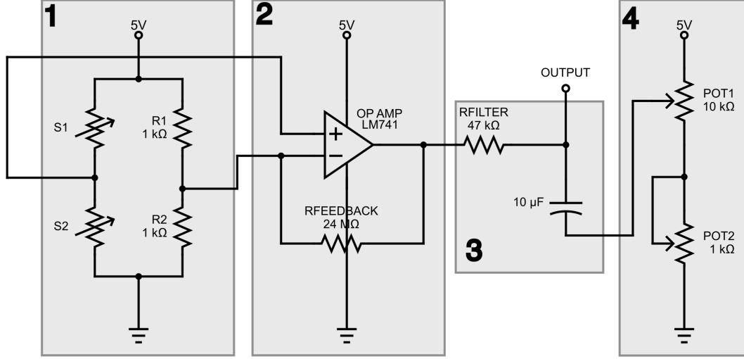
Figure 3.13: Circuit developed for the torque measurement setup, following the design principles of Chiu et al. (2016)[58]. Features include, 1. half Wheatstone Bridge Strain Gauge, 2. Amplifier, 3. Low-pass filter, 4. Coarse-fine adjustable reference network.
