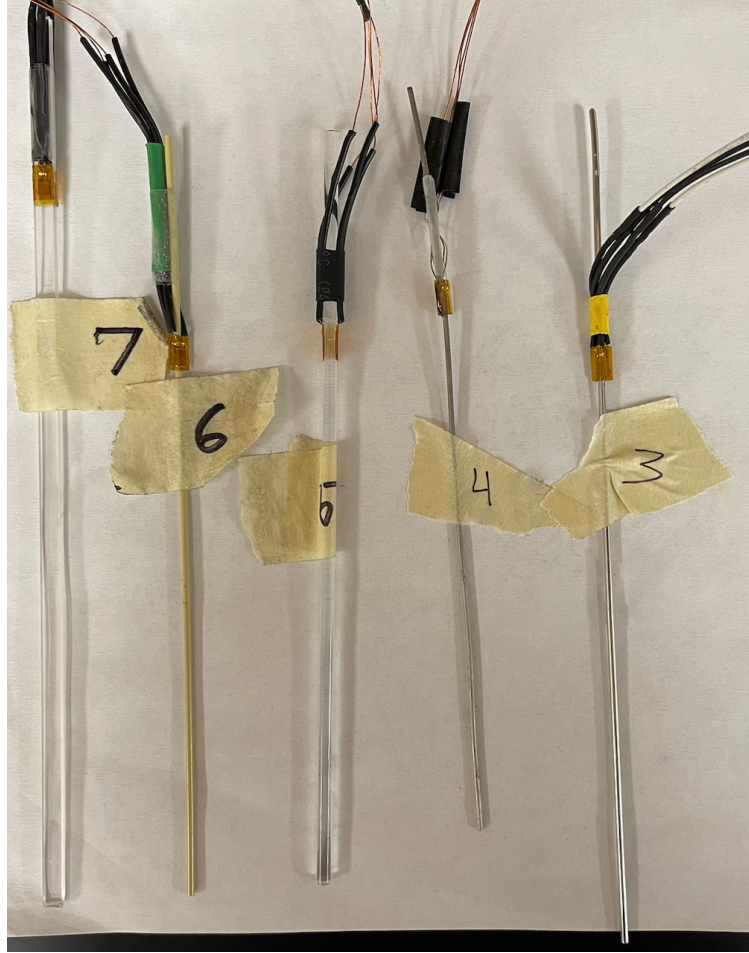
Figure 3.12: Rods fabricated during the torque experiment design. From left to right, (7) Clear Plastic, (6) Yellow plastic 2 , (5) Glass, (4) Titanium 1 , (3) Aluminum
