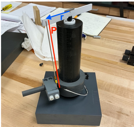
(a) Main torque fixture pole. Key adjustable parameters for maximizing measured torque are the sensor's tip position P (red) and the distance from center to sensor along the transfer arm r (blue).
