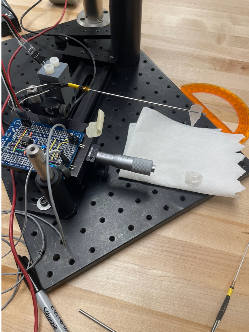
Figure 3.14: Circuit and sensor. The sensor was clipped with a custom made PVC clamp horizontally to act as a cantilever beam, a boat at length L was added, then a pipette was used to add water and see voltage changes with weight.
