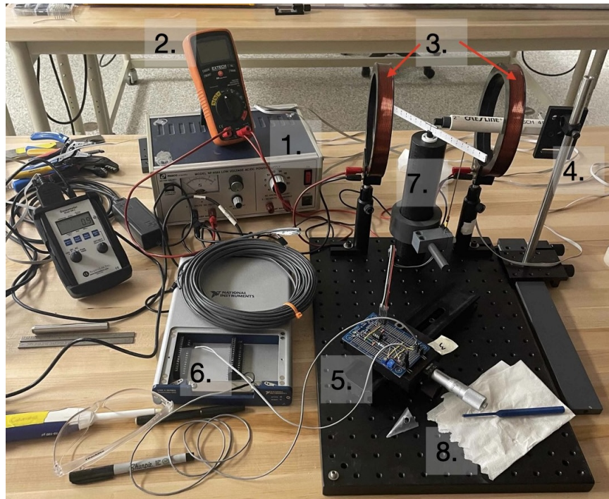
Figure 3.15: Experimental setup for torque. Includes magnetic field generation and measurement devices, 1 through 4. 5 is the circuit explained in section 3.3.3.2, 6. is a Data Acquisition (DAQ) system connected to a laptop and 7. is the main device where the dowel subject sits.
