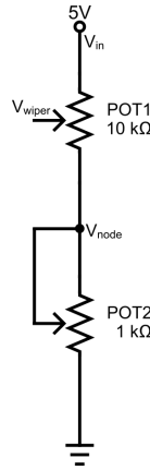
Figure B.2: Schematic of the coarse-fine potentiometer configuration used for the voltage-divider derivations in Figure 3.13.
