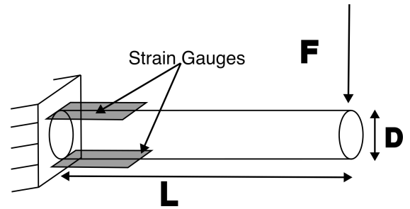
Figure 3.11: Cantilever setup showing the fixed cylinder and strain gauges "sandwiching" the rod at its base.
