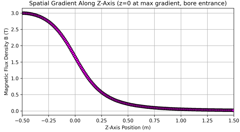
Figure 2.6: Expected 1D axial magnetic field B_z for an ideal solenoid, mimicking an MRI scanner.
