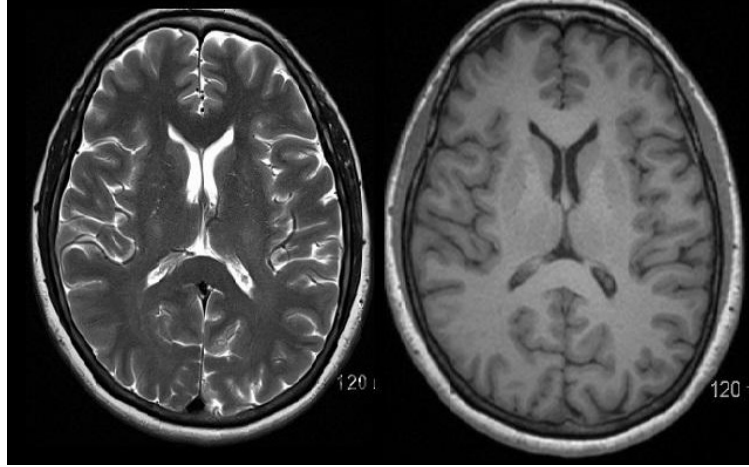
Figure 2.3: Comparison between T1- and T2-weighted brain MRI images of the same subject. The left image shows a T2-weighted scan, where cerebrospinal fluid (CSF) appears bright, and the right image shows a T1-weighted scan, where fat and white matter appear bright. Adapted from [31].
