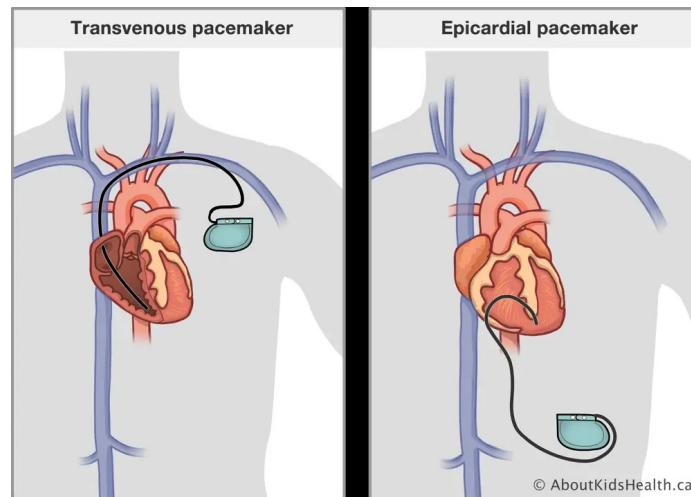
Figure 2.10: Comparison of transvenous vs epicardial lead placement in pacemakers (adapted from [3]).
