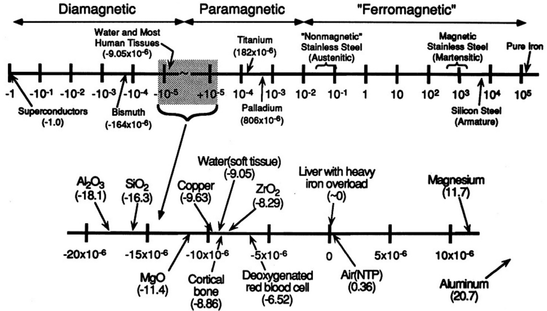
Figure 2.8: Spectrum of magnetic susceptibilities. The upper diagram uses a logarithmic scale to indicate the full range of observed magnetic susceptibility values: it extends from -1.0 for superconductors to 100,000 for soft ferromagnetic materials. The bottom diagram uses a linear scale (in ppm) to indicate the properties of some materials with 20 ppm. The susceptibilities of most human tissues are in the range from 7.0 to 11.0 ppm. Adapted from Schenck [16].
