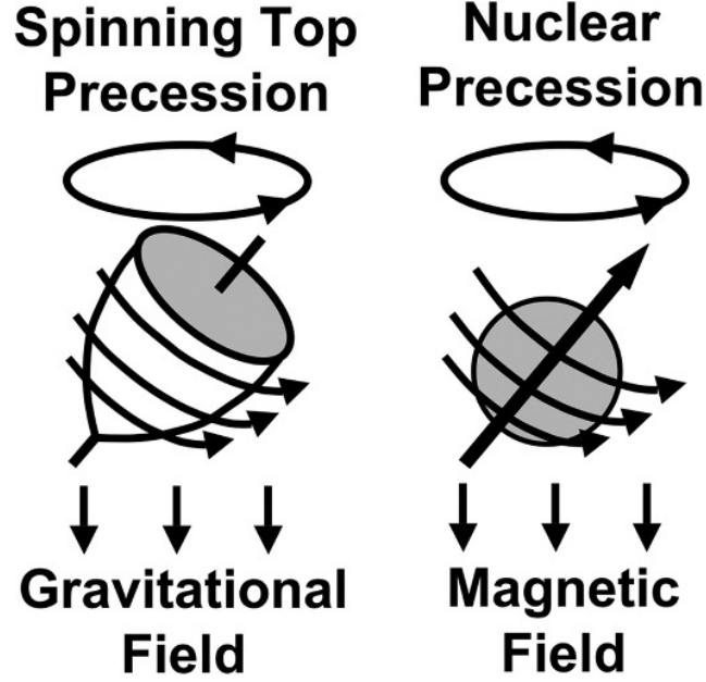
Figure 2.2: Illustration of proton precession under a static magnetic field B_0 compared to that of a spinning top under gravity. Adapted from Pooley, R. A., Fundamental physics of MR imaging , (2005) [1].
