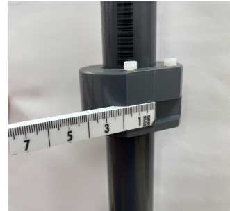
(c) Lower ring close-up with horizontal 20 cm ruler.
