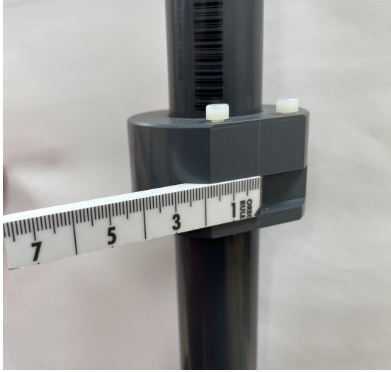
(a) PVC-based mapping platform.
