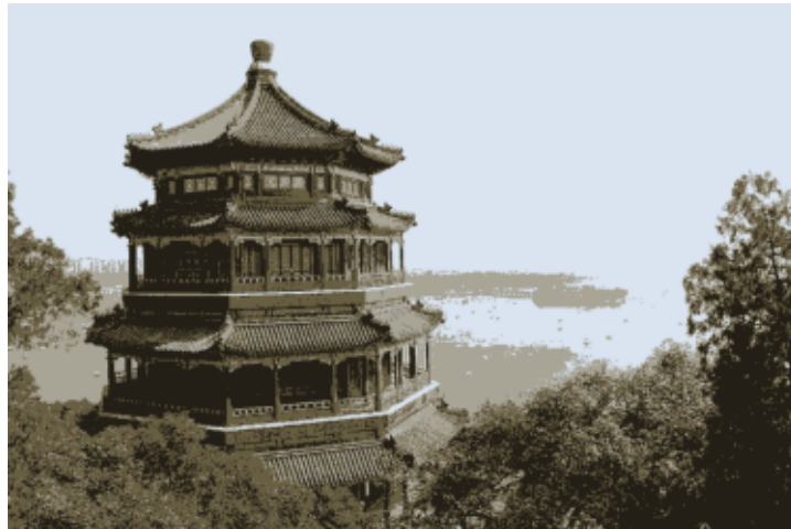
K = 4 MSE = 456.36
