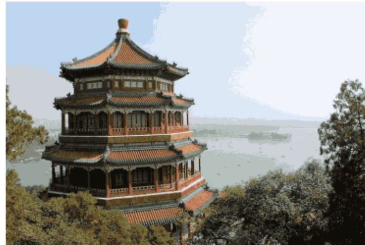
K = 16 MSE = 115.14
