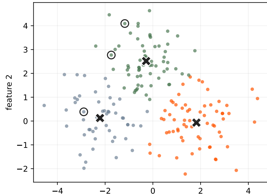
random A final SSE = 295.6, 6 iterations
