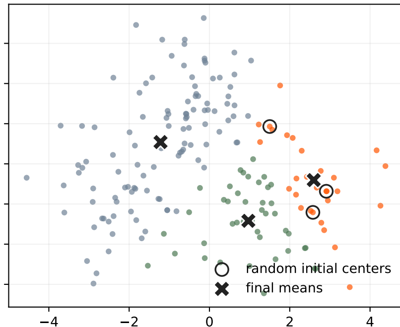
random B final SSE = 506.4, 6 iterations
