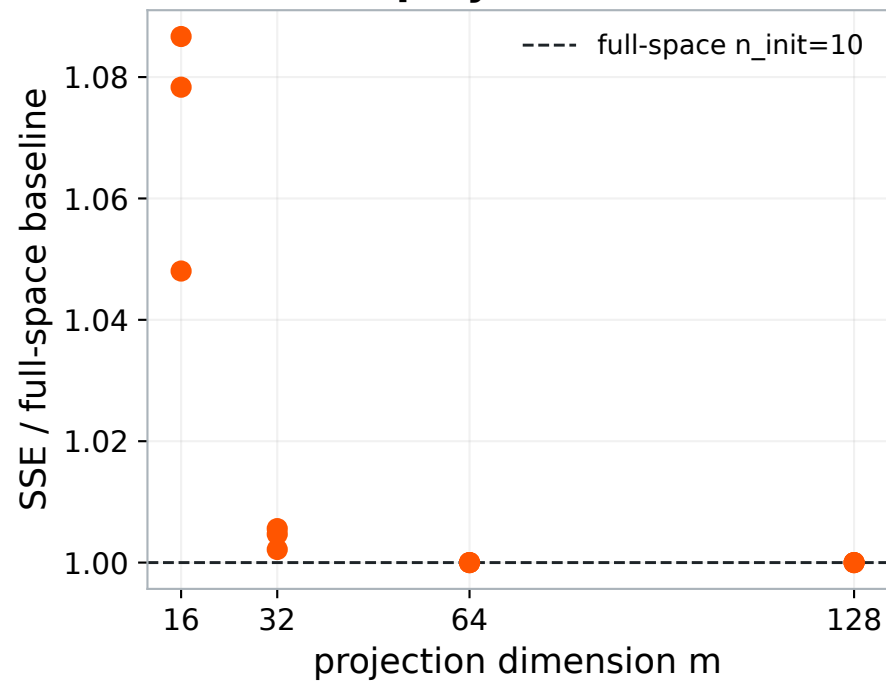
Original-space SSE from projected labels
