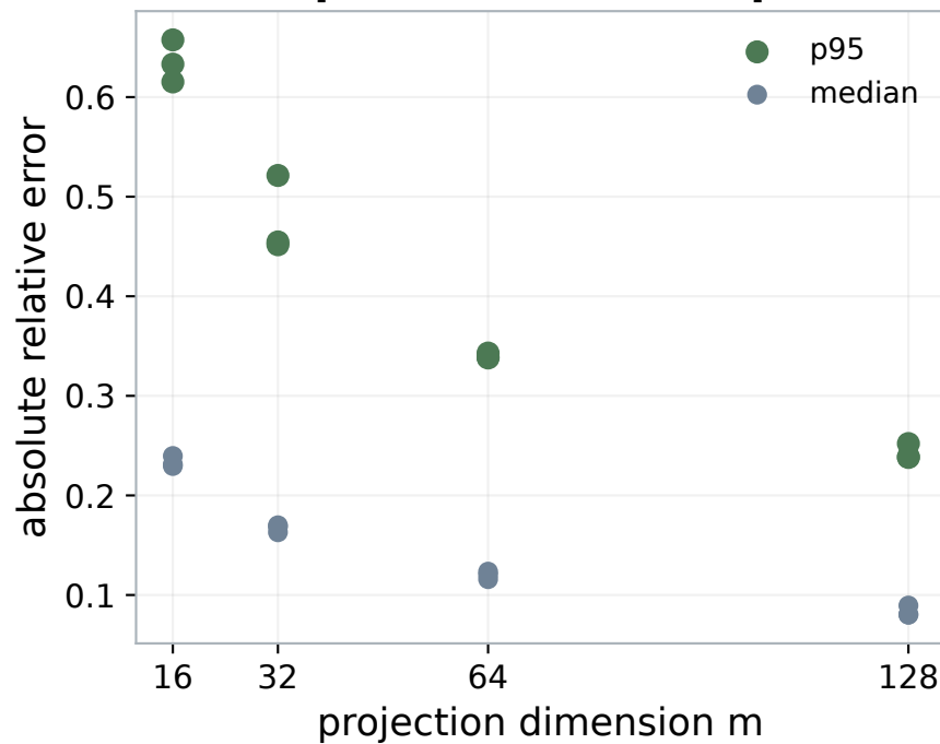
JL pairwise distortion 600 points \rightarrow 179,700 pairs
