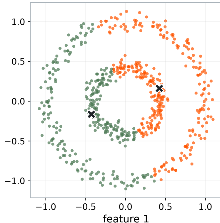
Concentric circles K-means ARI = -0.002
