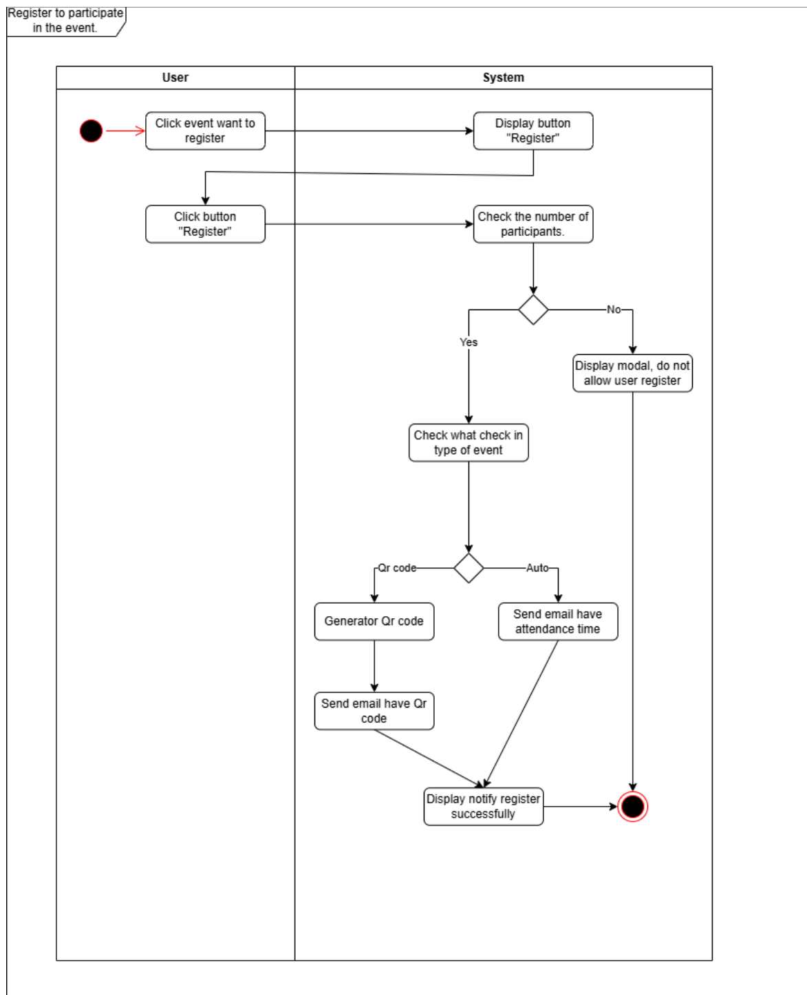
Figure 4.2. Activity diagram register the event
