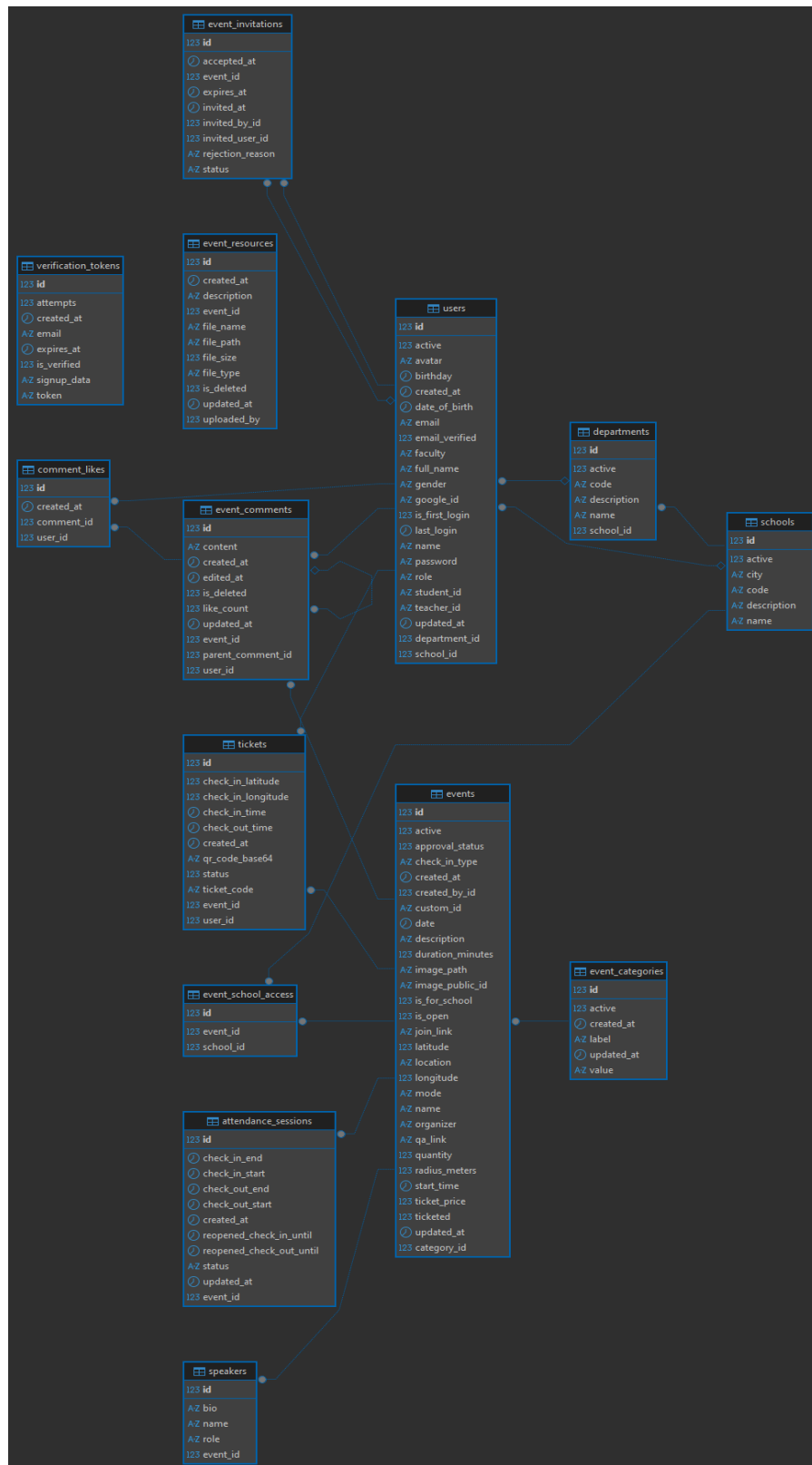
Figure 5.1. Entity relation diagram
