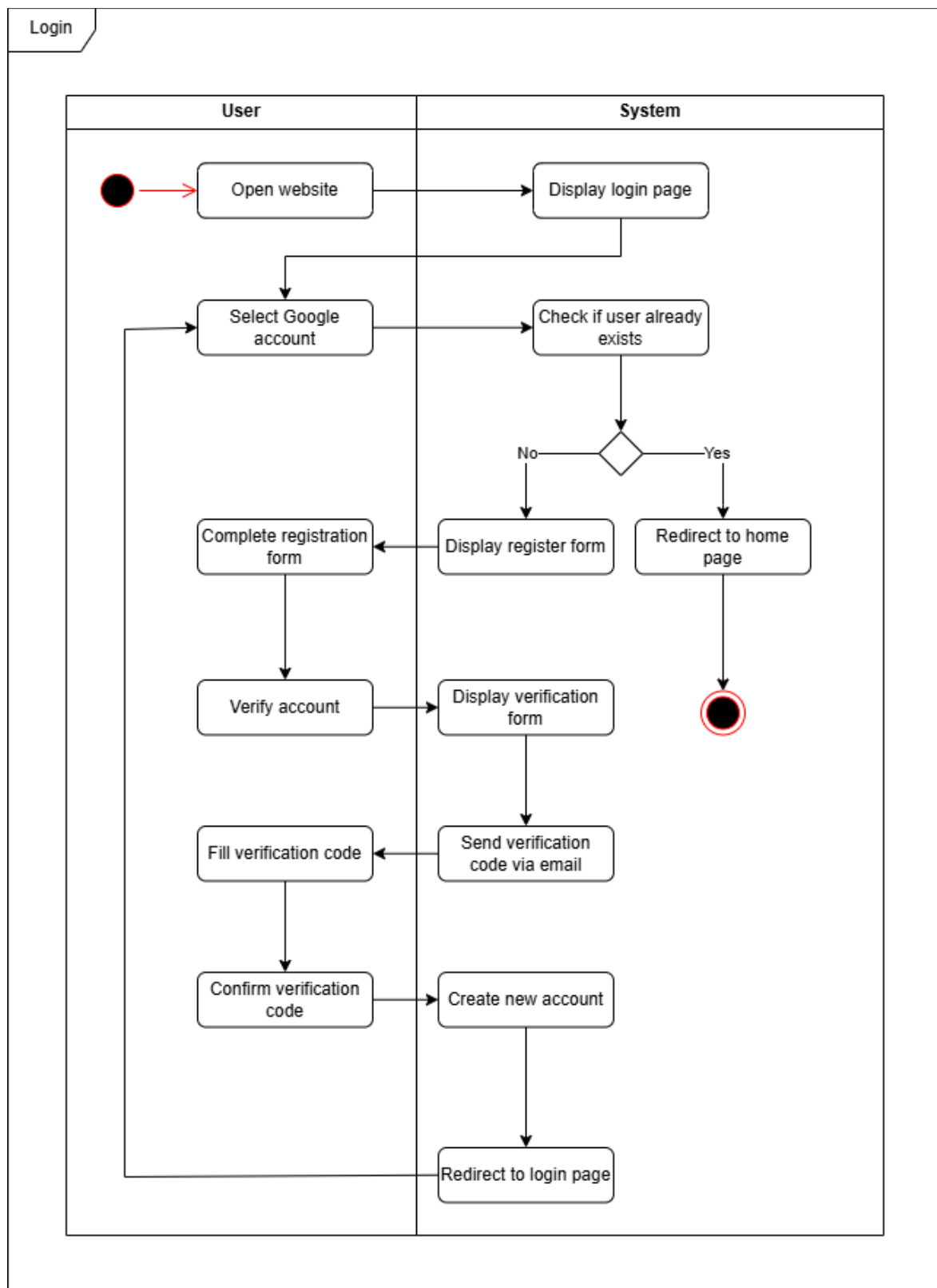
Figure 4.1. Activity diagram login
