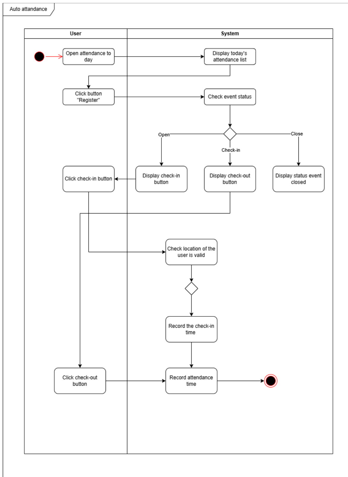
Figure 4.3. Activity diagram auto attendance
