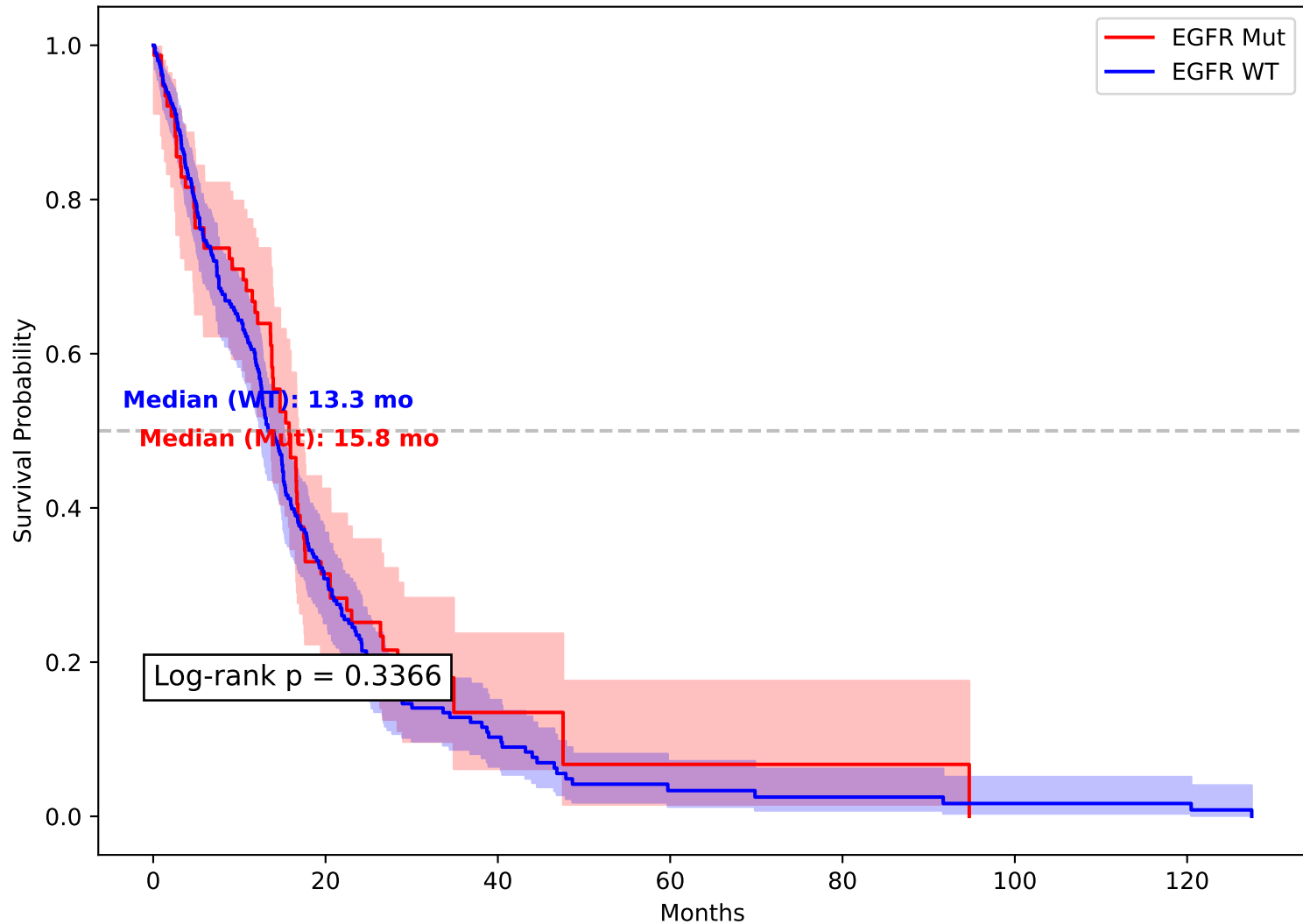
EGFR Survival in GBM (p=0.3366)
