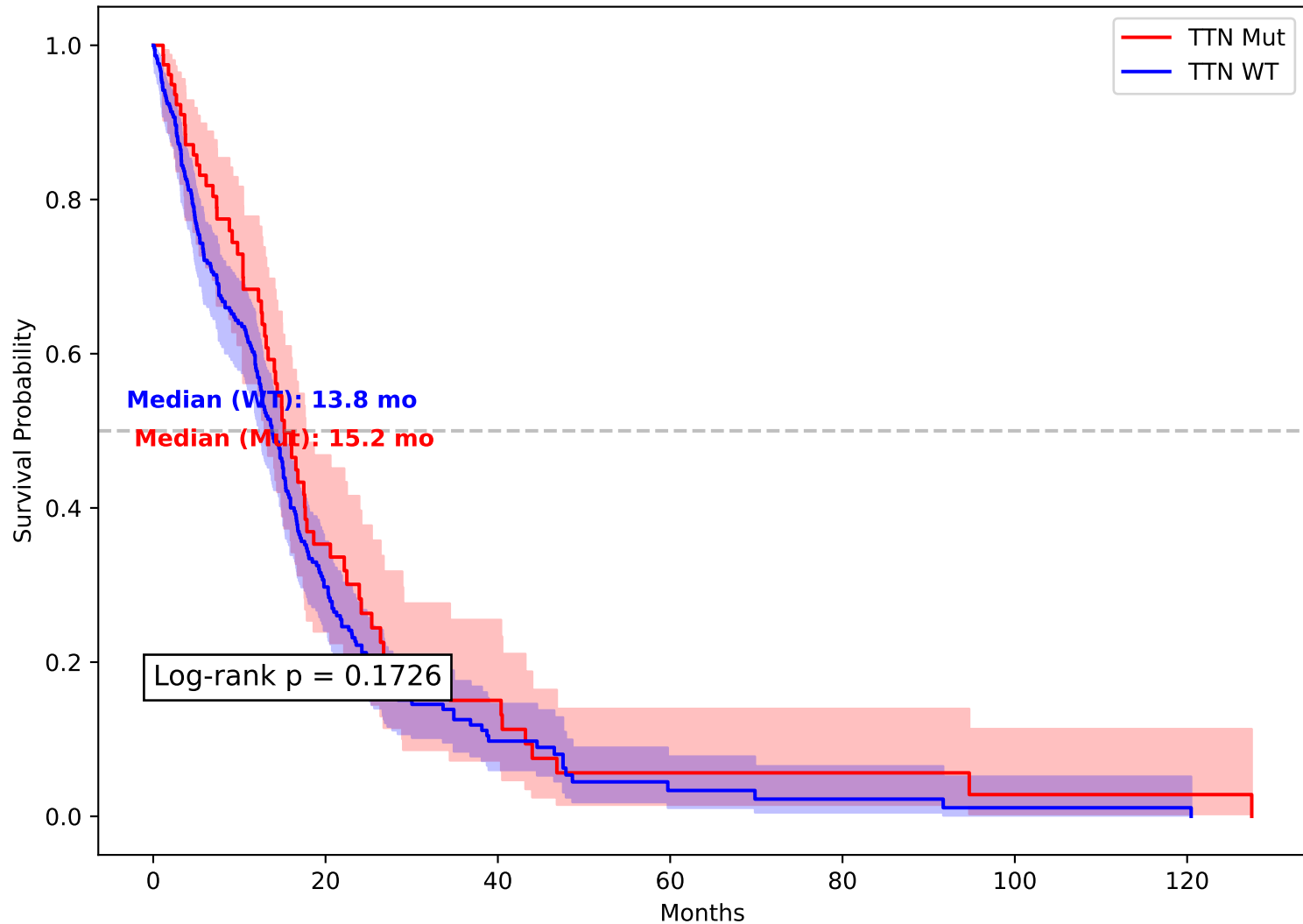
TTN Survival in GBM (p=0.1726)
