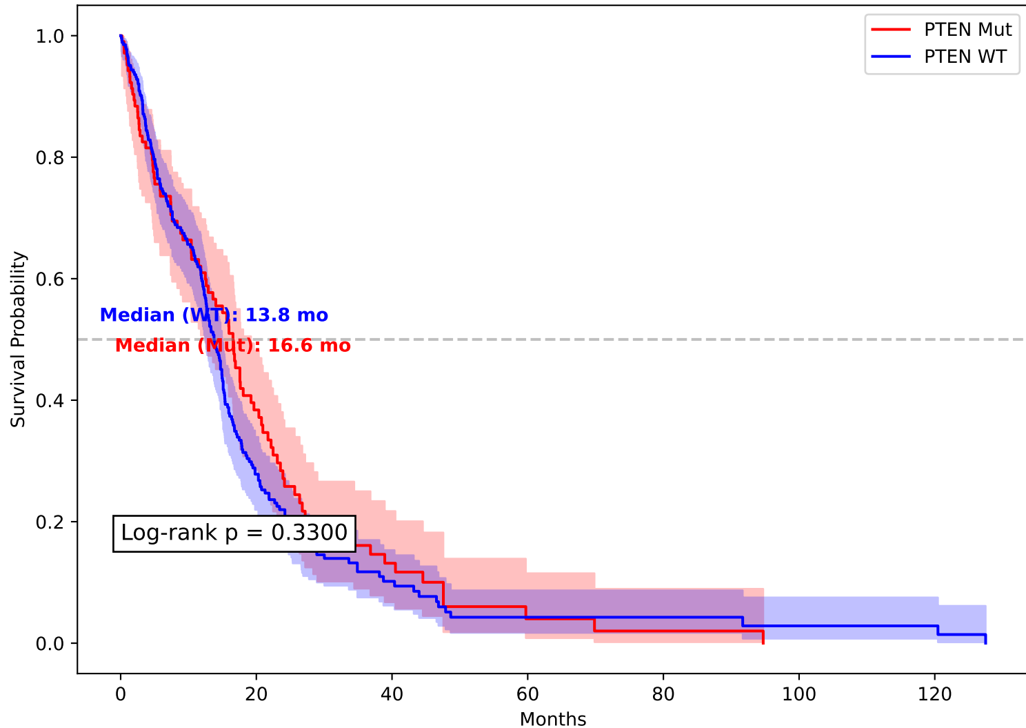
PTEN Survival in GBM (p=0.3300)
