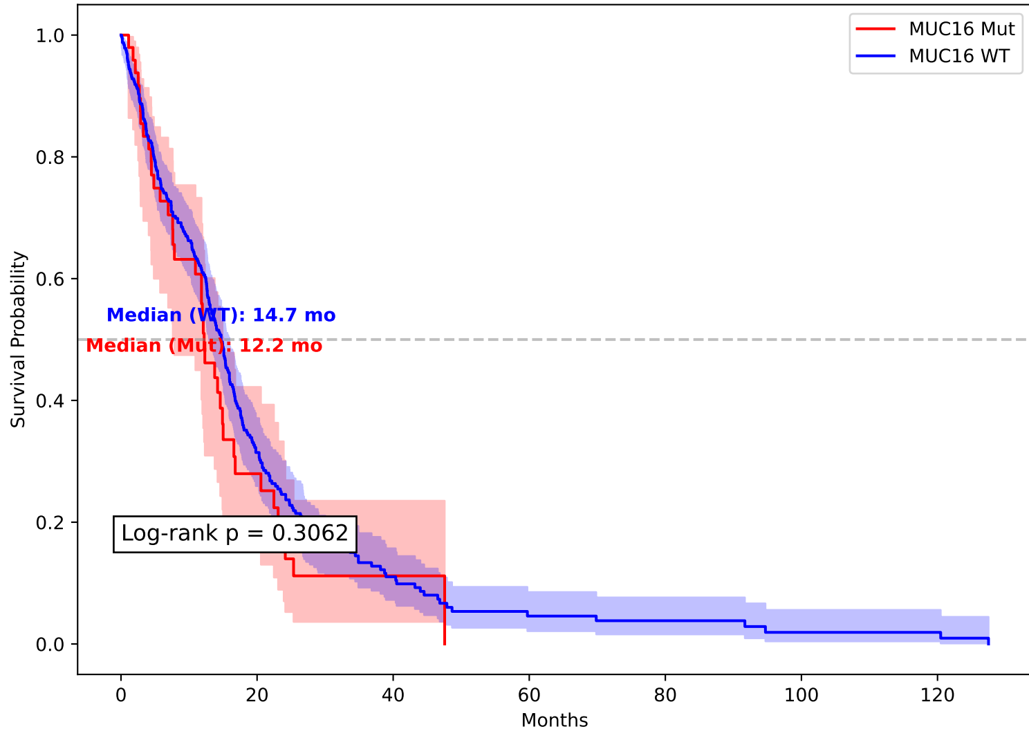
MUC16 Survival in GBM (p=0.3062)
