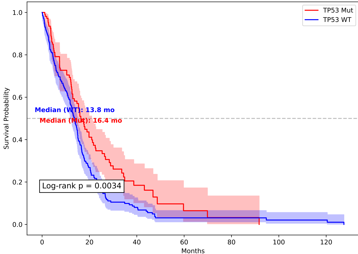
TP53 Survival in GBM (p=0.0034)
