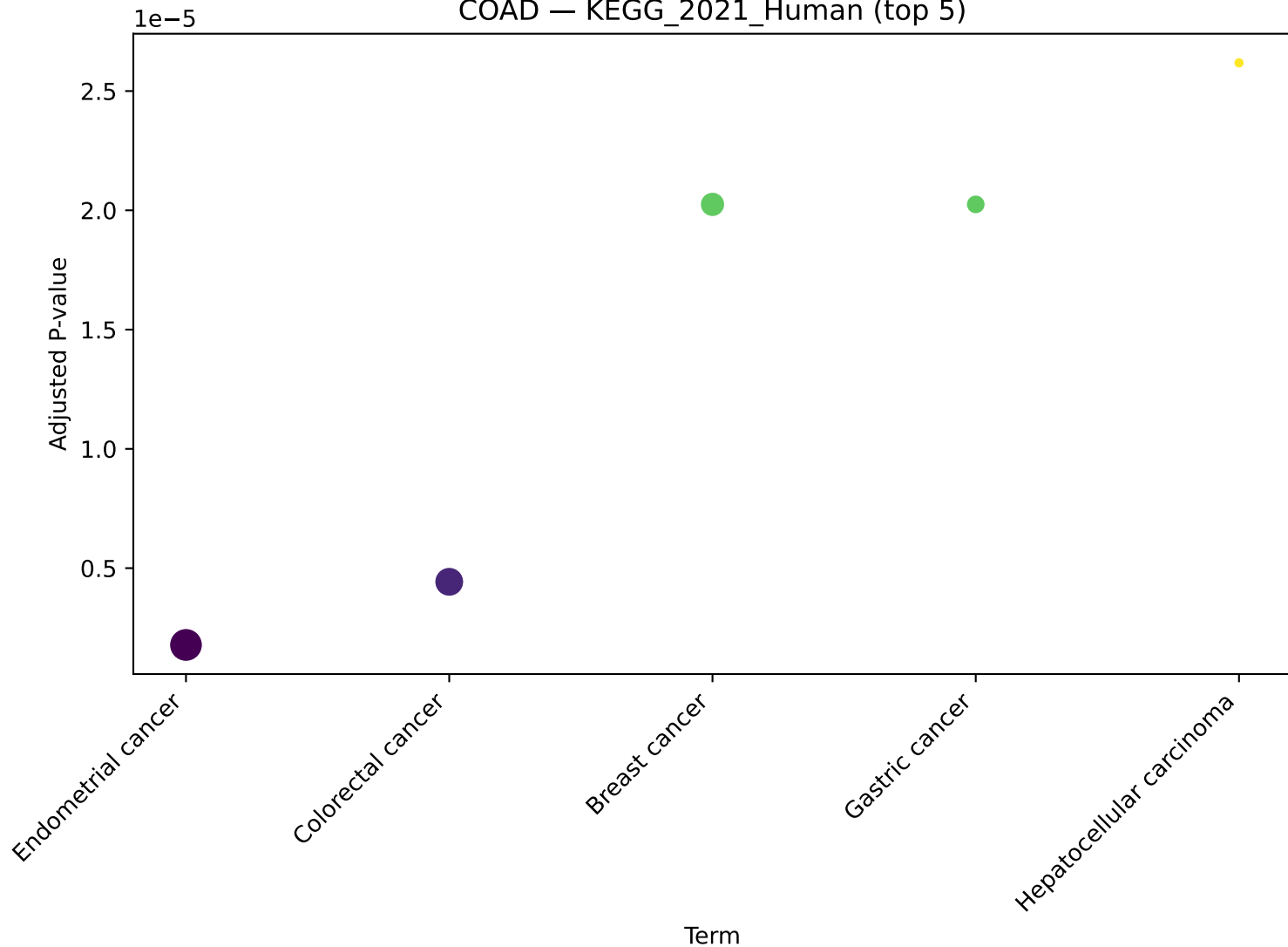
COAD — KEGG_2021_Human (top 5)
