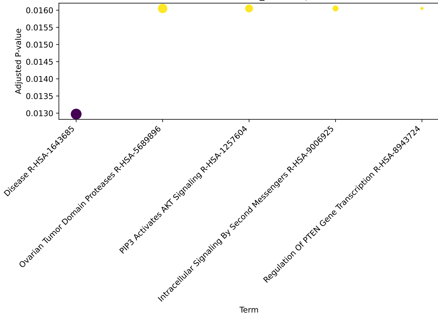
GBM — Reactome_2022 (top 5)
