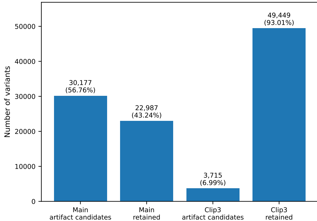
GBM main vs clip3 sensitivity
