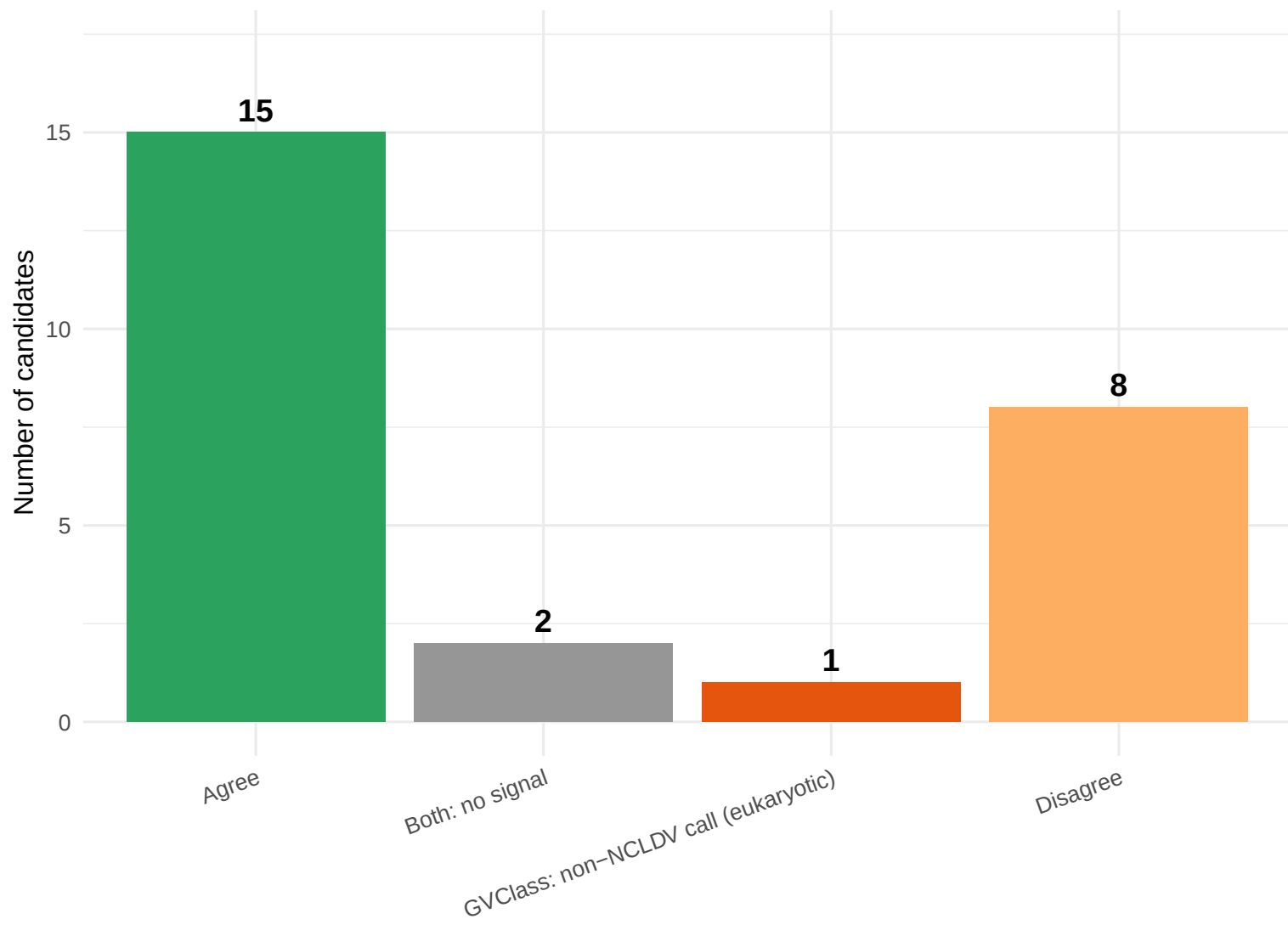
TIGTOG vs. GVClass taxonomic agreement across 26 candidates
