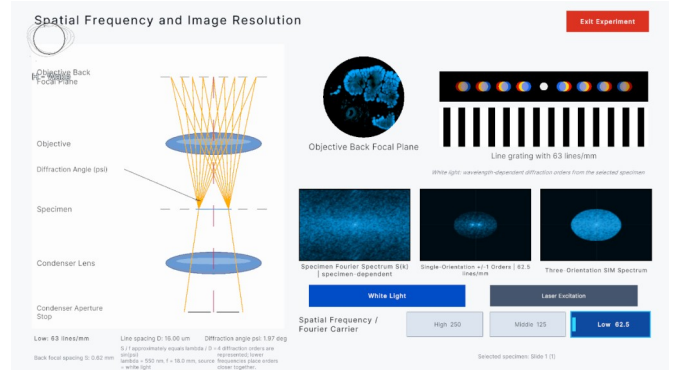
Fig. 2. Mapping instructional inputs to observable feedback. Focus, NA, and illumination carrier affect specimen display, cone geometry, and sideband/support displays, respectively. The feedback combines authored mappings and simplified numerical visualization; the captures identify the changed input rather than claiming calibrated optical measurements.
