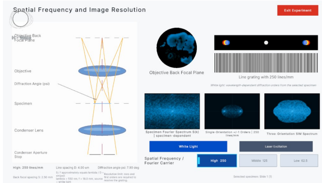
Fig. 2. Mapping instructional inputs to observable feedback. Focus, NA, and illumination carrier affect specimen display, cone geometry, and sideband/support displays, respectively. The feedback combines authored mappings and simplified numerical visualization; the captures identify the changed input rather than claiming calibrated optical measurements.
