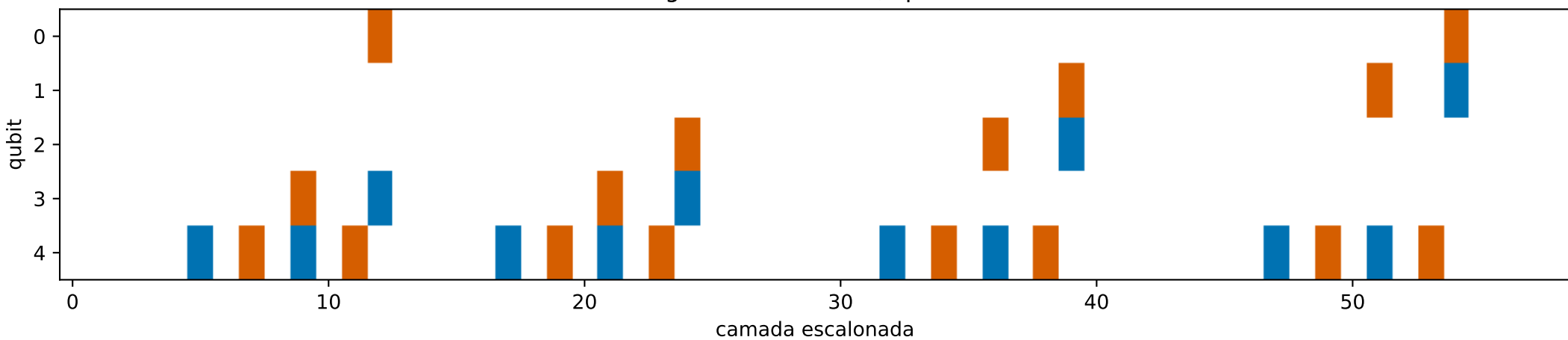
PyZX: T-count=8, span=31
