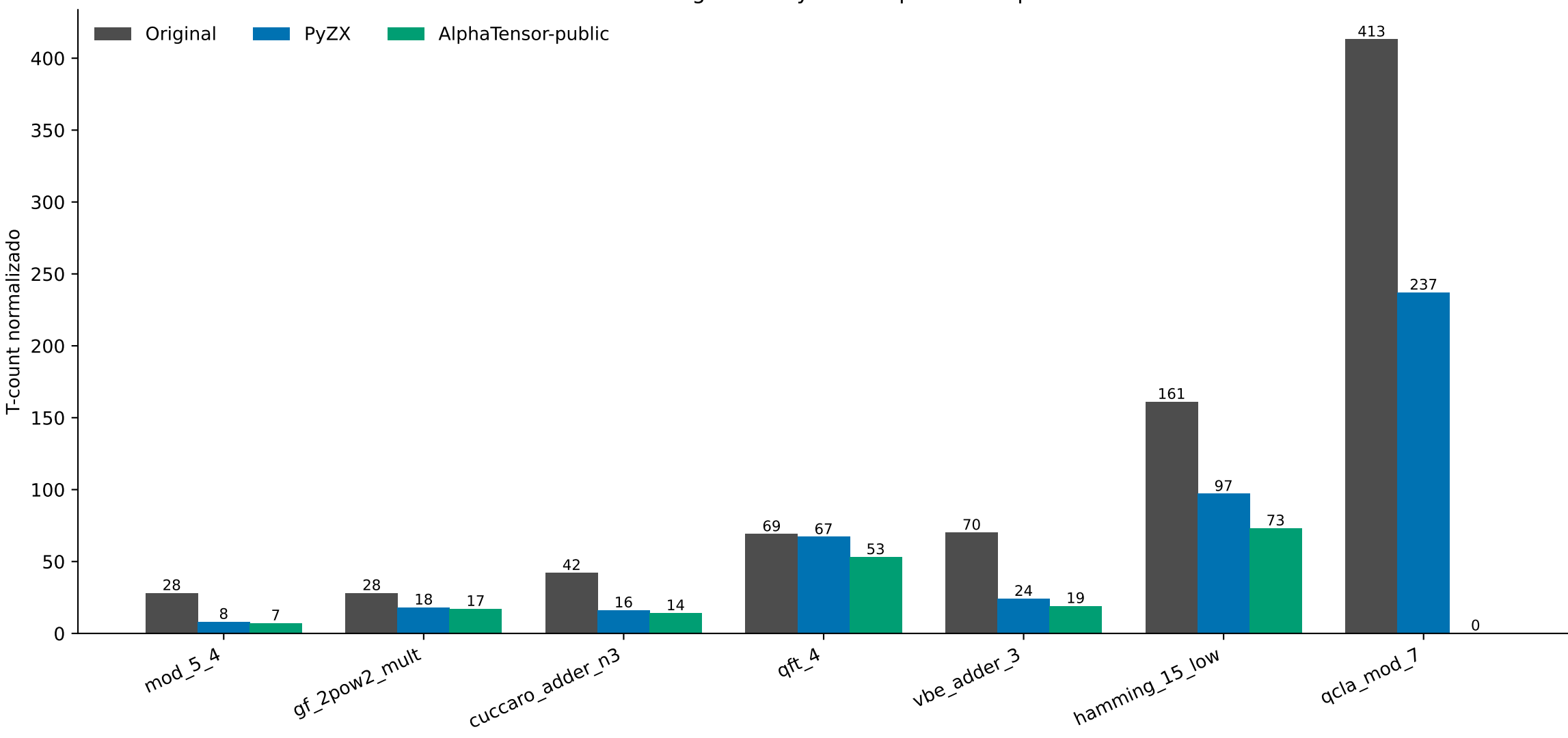
T-count: Original vs PyZX vs AlphaTensor-public
