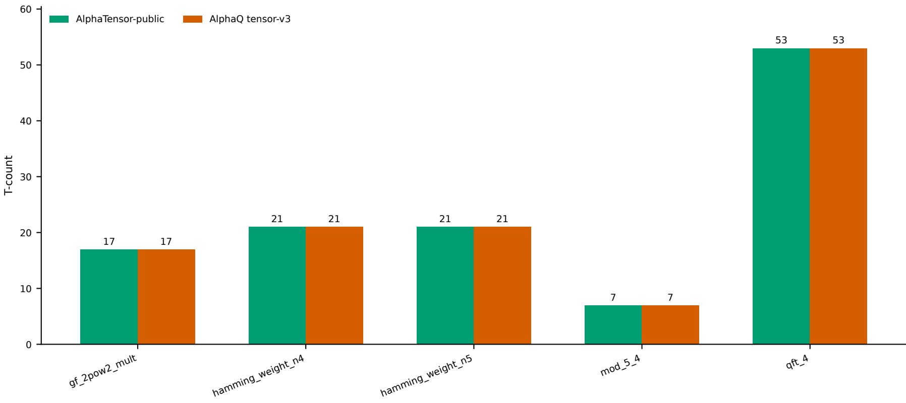
T-count: public baseline vs tensor-v3 selection
