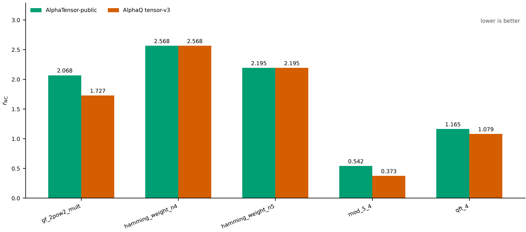
Primary non-Clifford-depth ratio
