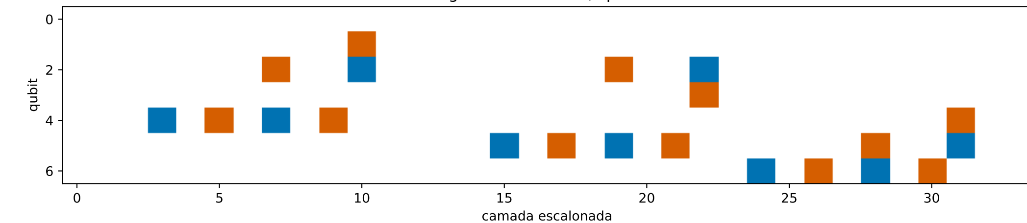
PyZX: T-count=21, span=None
