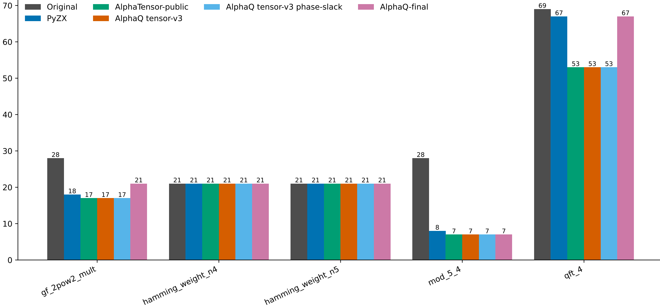
T-count: Original vs baselines vs AlphaQ tensor-v3
