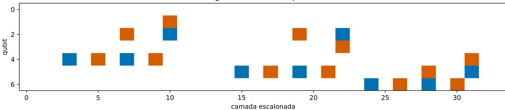
PyZX: T-count=21, span=84
