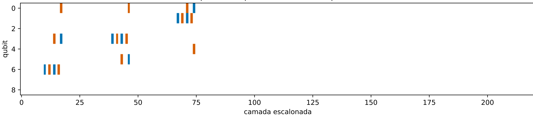
AlphaQ tensor-v3: T-count=21, span=65
