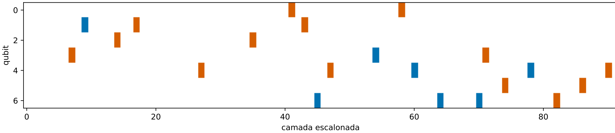
AlphaTensor-public: T-count=21, span=65
