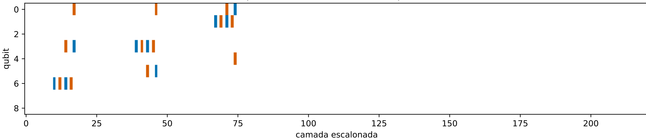
AlphaQ tensor-v3 phase-slack: T-count=21, span=65
