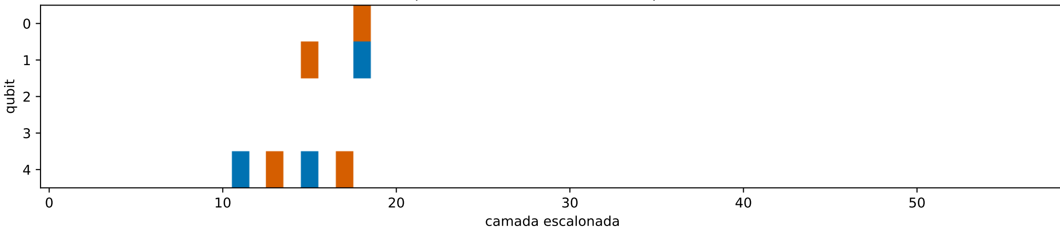
AlphaQ tensor-v3 phase-slack: T-count=7, span=8
