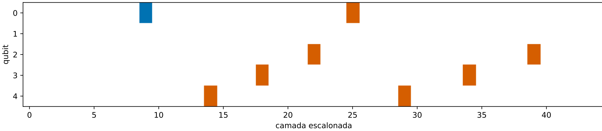
AlphaTensor-public: T-count=7, span=27
