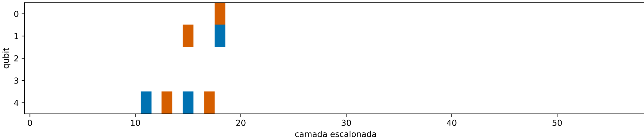
AlphaQ-final: T-count=7, span=8
