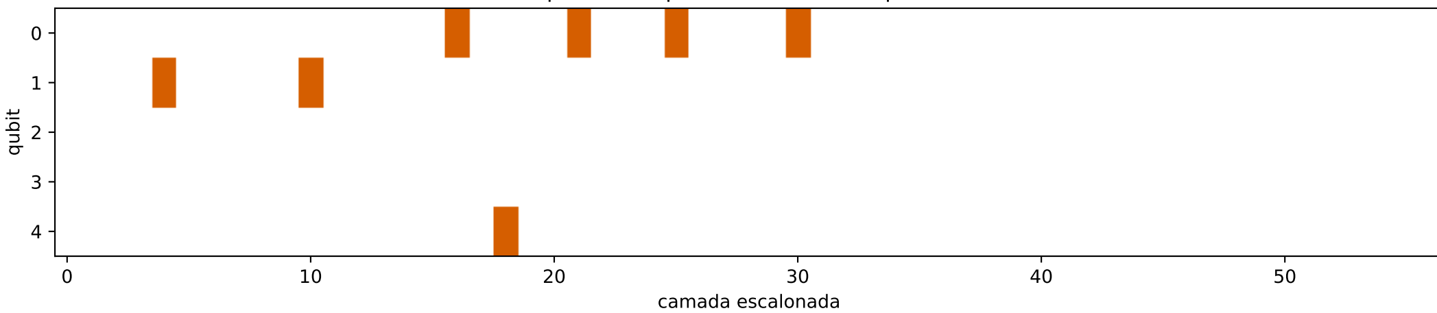
AlphaQ tensor-v3: T-count=7, span=8
