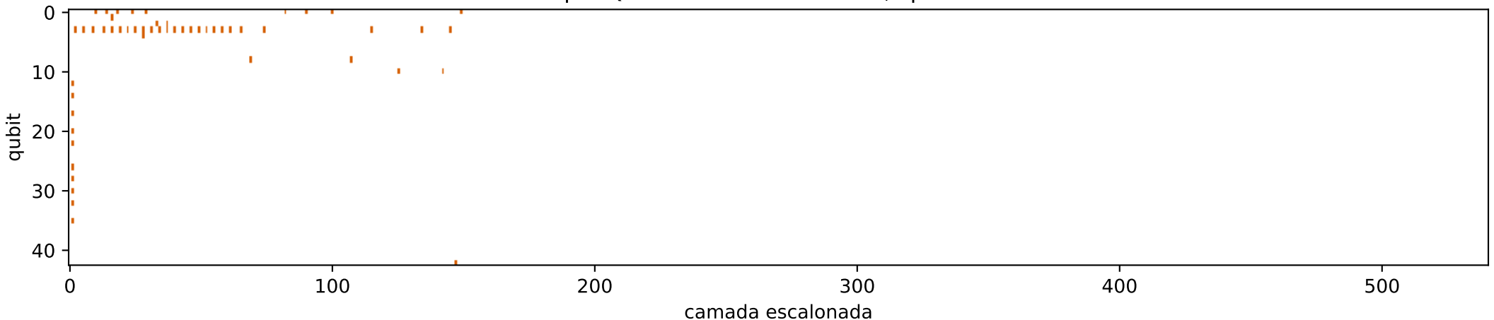
AlphaQ tensor-v3 phase-slack: T-count=53, span=136
