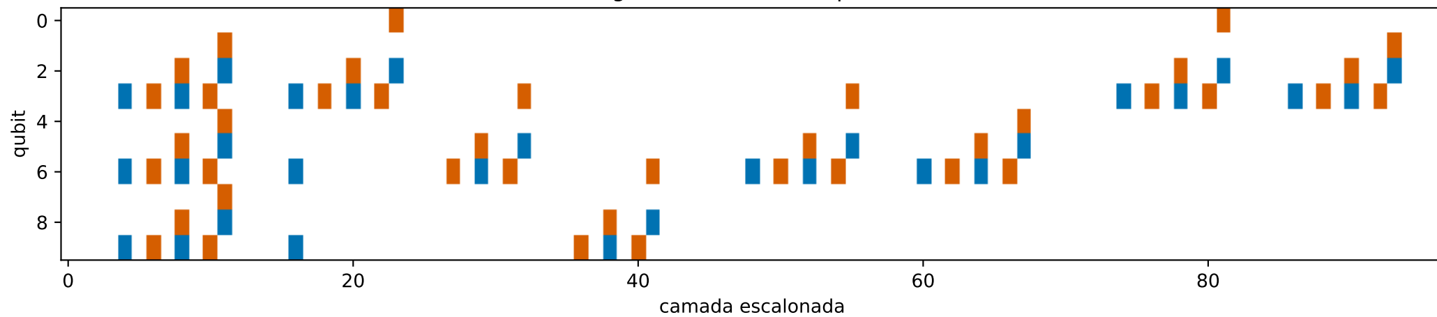
PyZX: T-count=24, span=106
