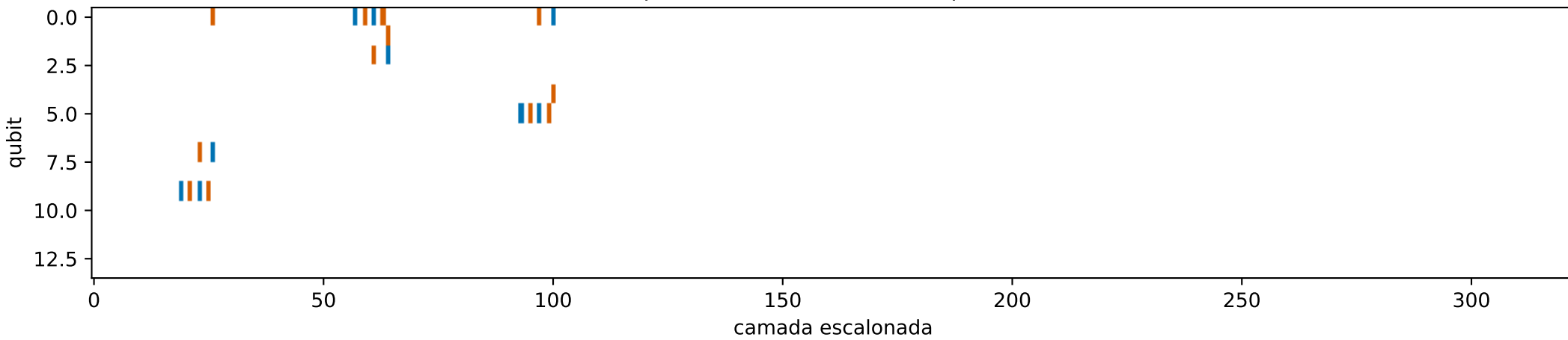
AlphaQ-final: T-count=21, span=82
