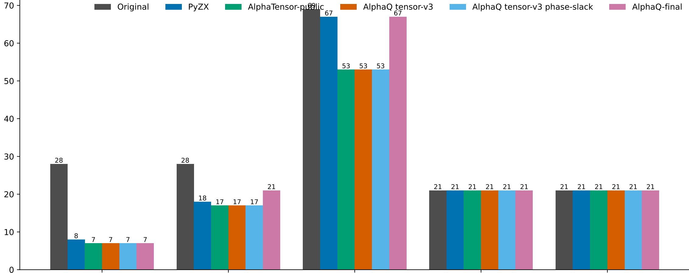
T-count: Original vs baselines vs AlphaQ tensor-v3
