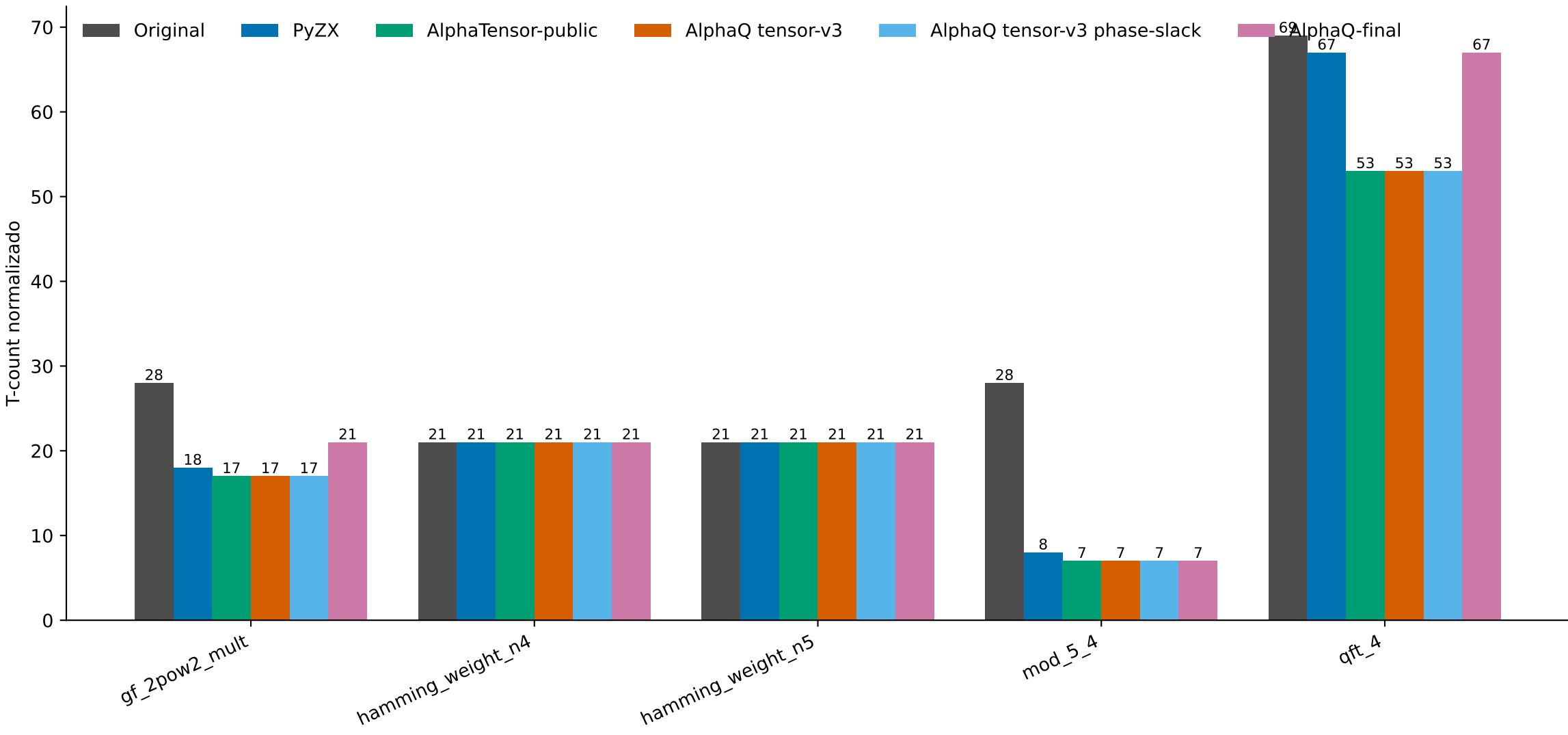
T-count: Original vs baselines vs AlphaQ tensor-v3
