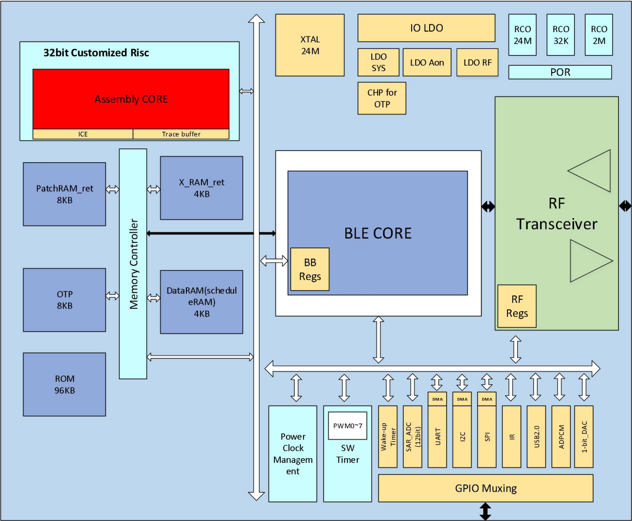
Figure 1- 1 Block diagram
