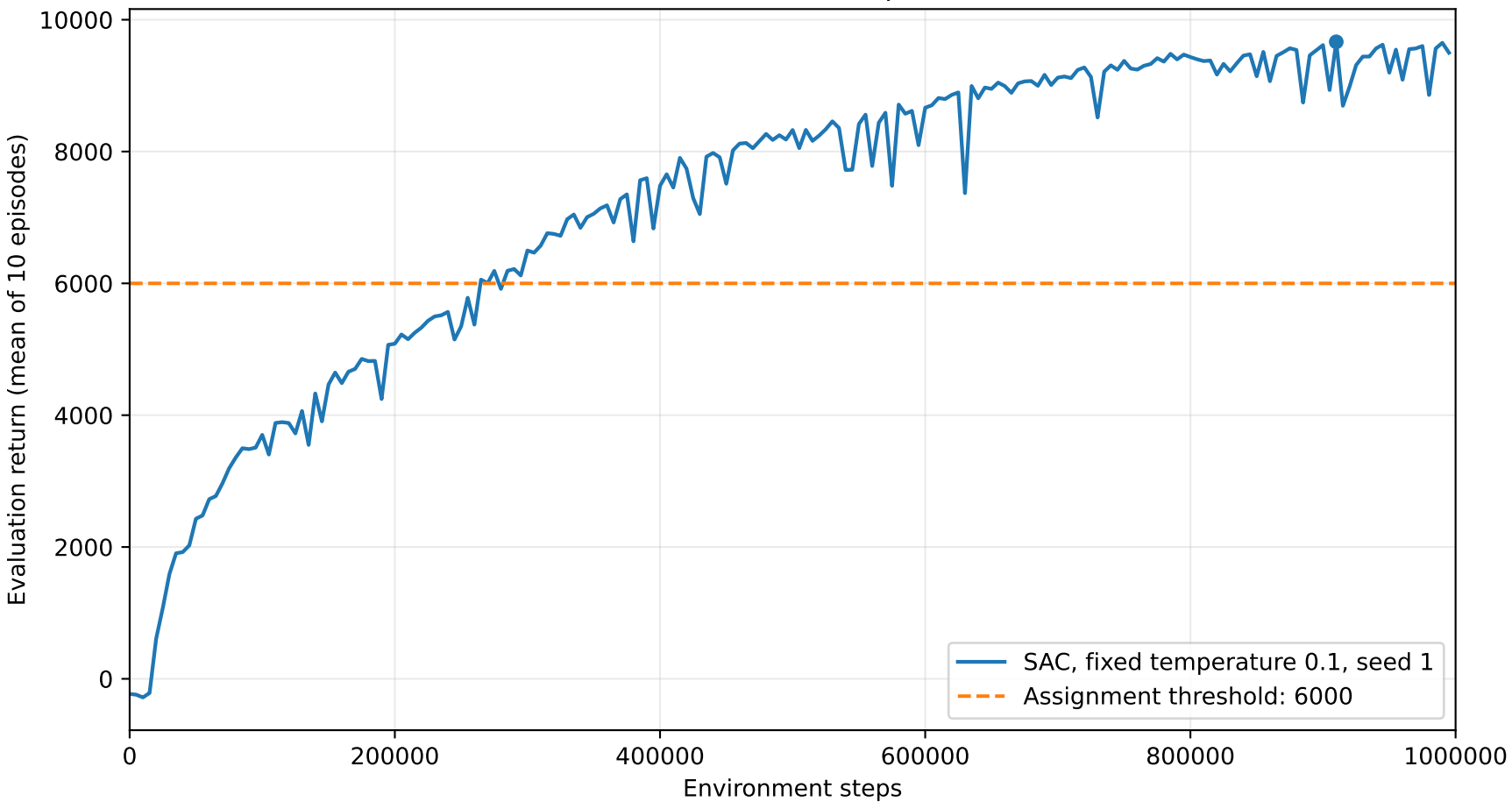
HalfCheetah-v4: fixed-temperature SAC
