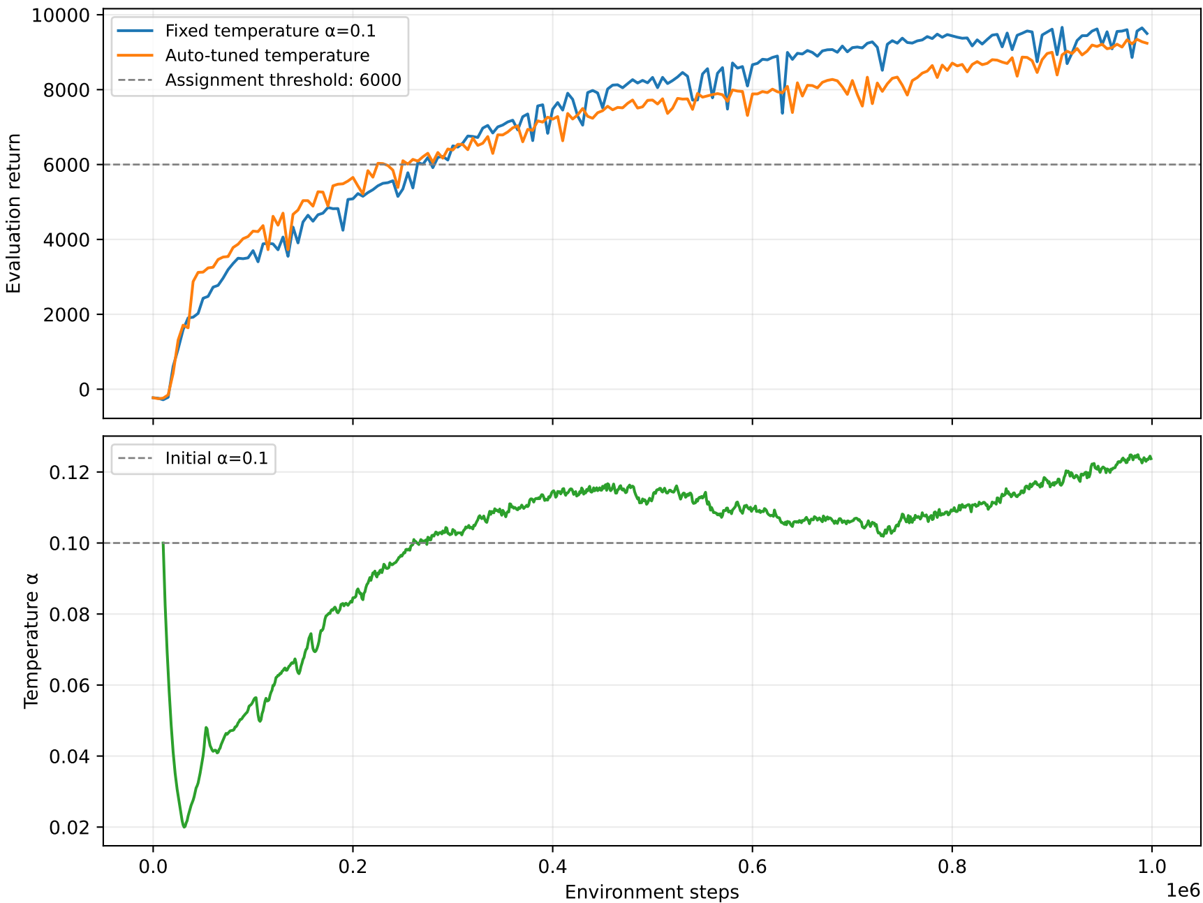
HalfCheetah-v4 SAC: fixed versus auto-tuned temperature
