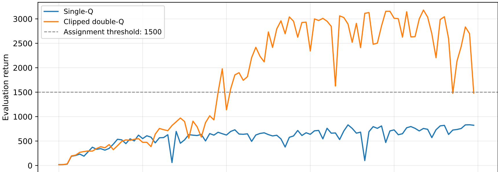
Hopper-v4 SAC: single-Q versus clipped double-Q
