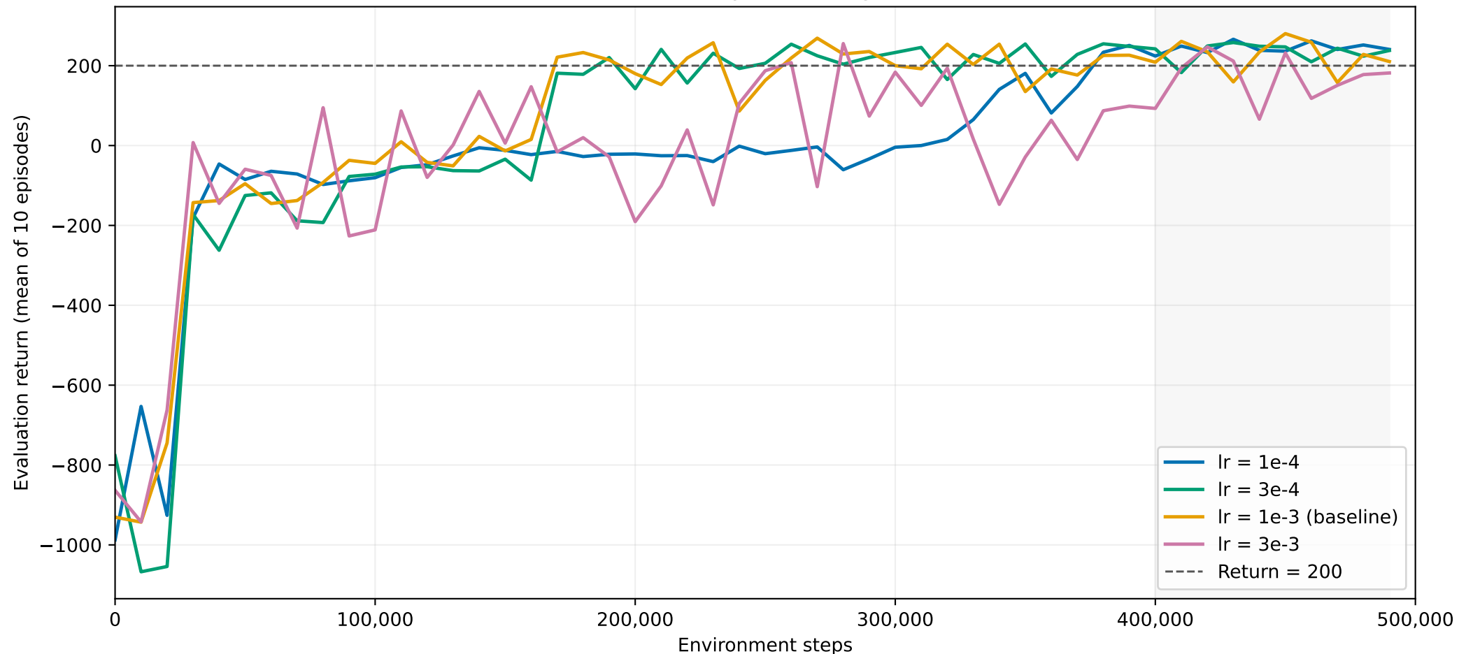
LunarLander-v2: sensitivity to learning rate (Double DQN)
