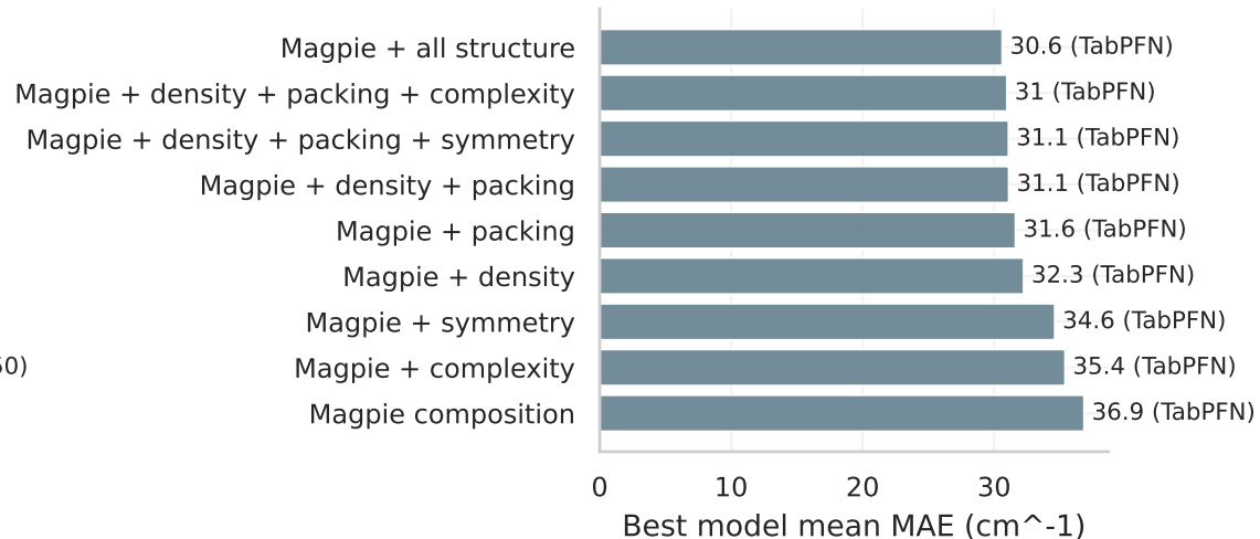
matbench_phonons
