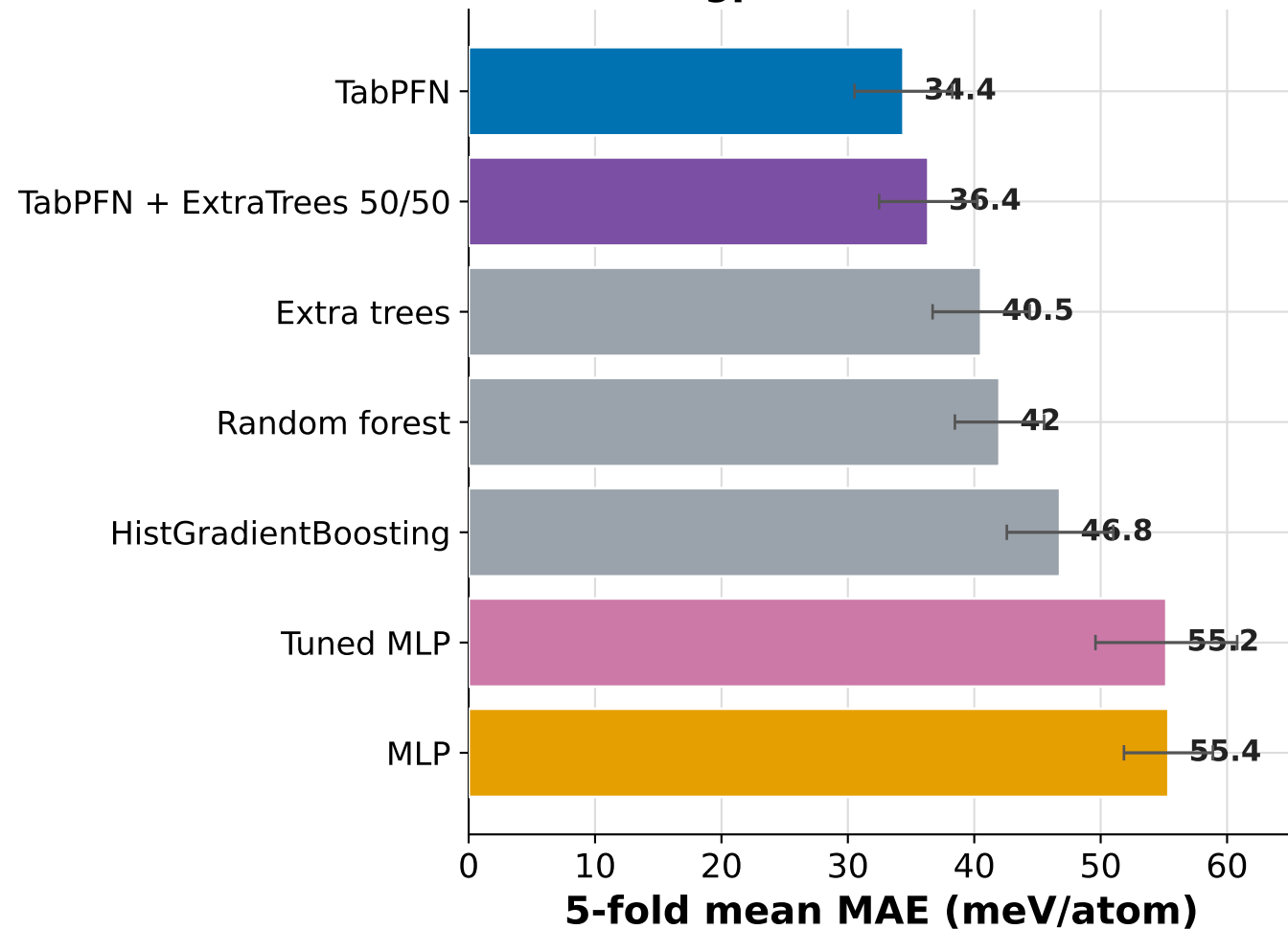
JDFT2D exfoliation energy (Magpie + all structure)
