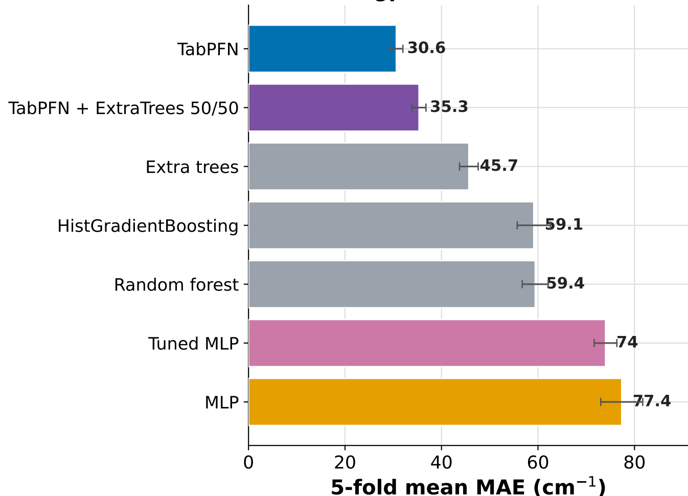
Phonon peak frequency (Magpie + all structure)
