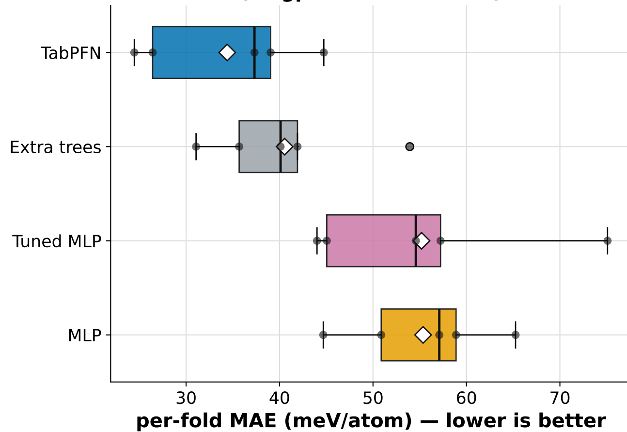
JDFT2D exfoliation energy (Magpie + all structure)
