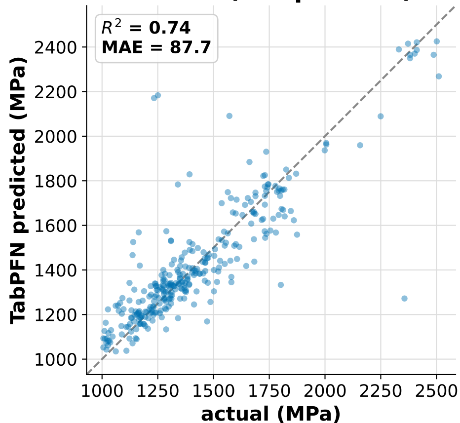
Steels (composition)
