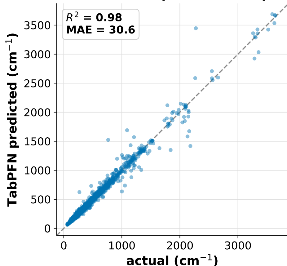
Phonons (+ structure)
