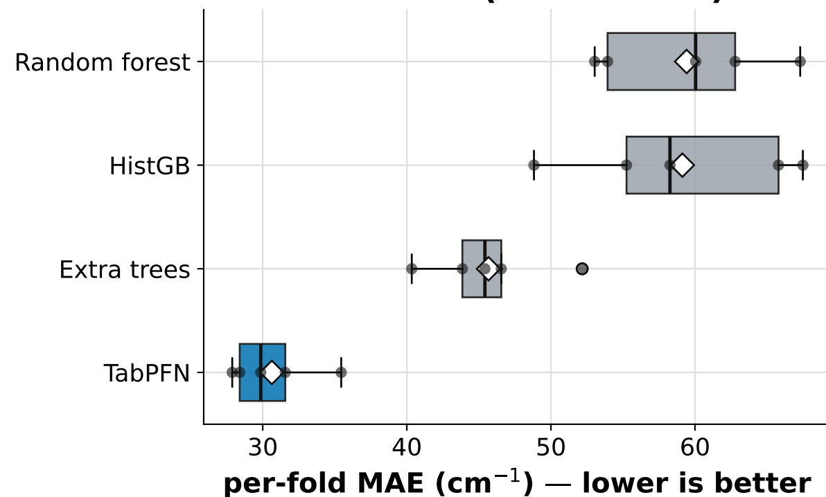
Phonons (+ structure)
