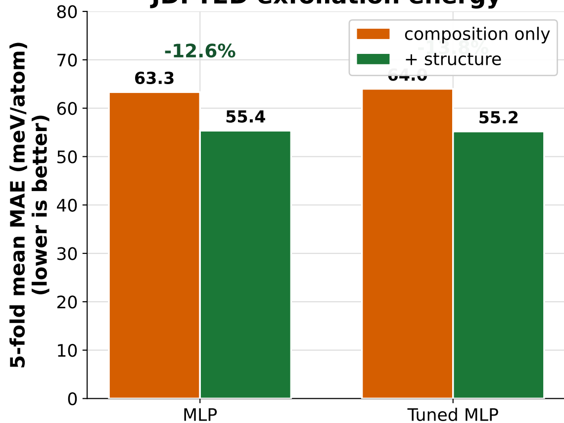
JDFT2D exfoliation energy
