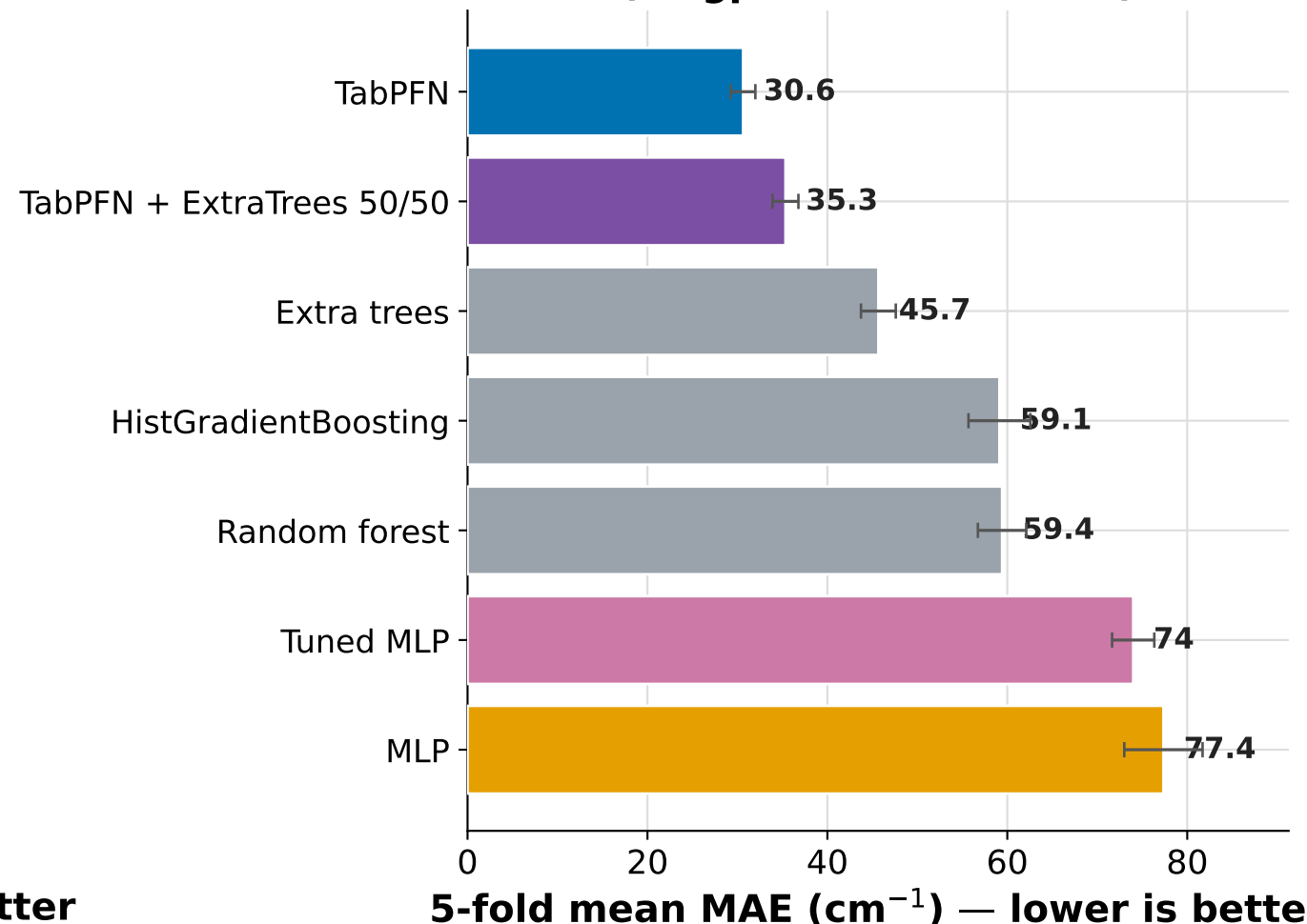
Phonon peak frequency (Magpie + all structure)
