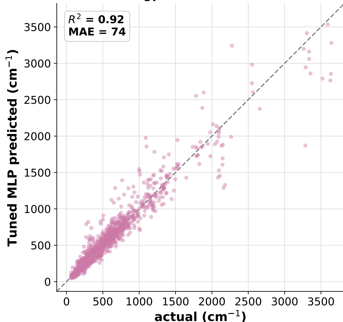
Phonon peak frequency (Magpie + all structure)
