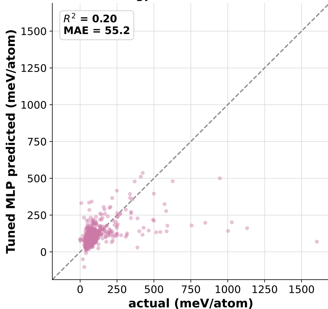
JDFT2D exfoliation energy (Magpie + all structure)
