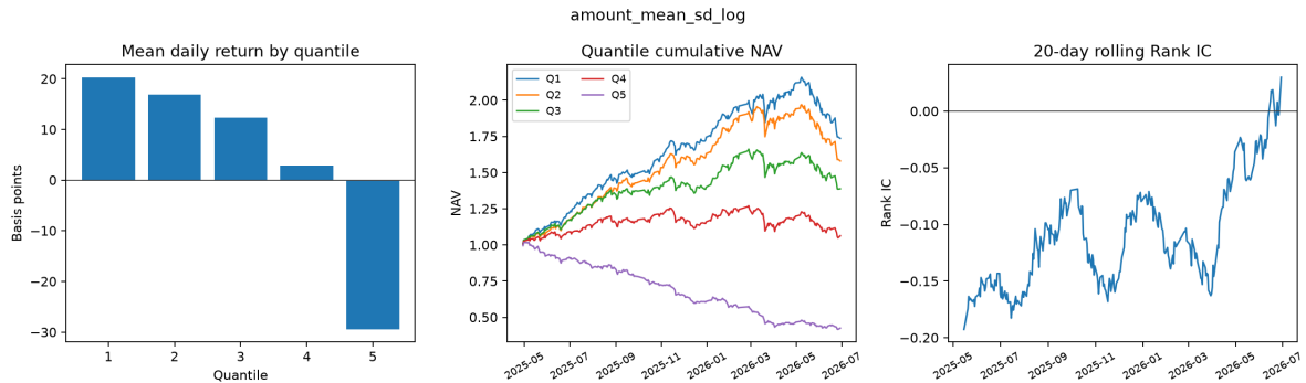
Figure 4.1: Diagnostics for the multi-window dispersion of average turnover. The negative Rank IC and declining portfolio returns indicate that this factor should be used with its sign reversed.
