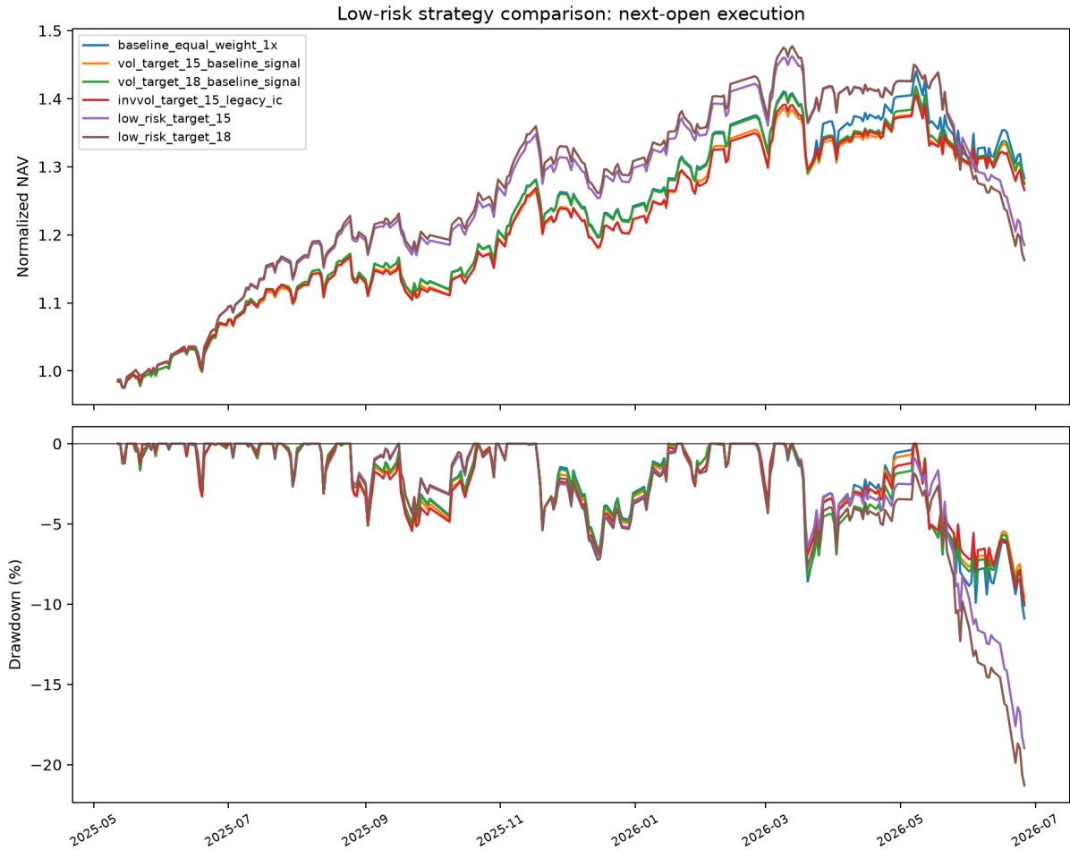
Figure 6.3: Net-value and drawdown decomposition across risk-control versions. Replacing the full factor and IC-weighting system lowers volatility but worsens holdout drawdown; the adopted version preserves the original signal and applies the 15% volatility target.
