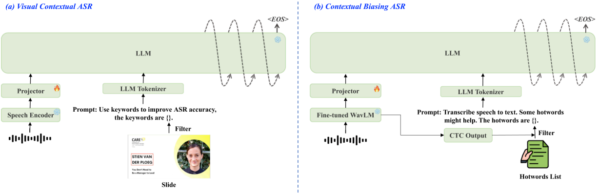
Fig. 3. (a) LLM-based Visual Contextual ASR in SLAM-LLM framework. (b) LLM-based Contextual Biasing ASR in SLAM-LLM framework.
