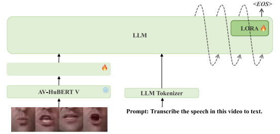
Fig. 4. The model architecture of LLM-based visual speech recognition (VSR) in SLAM-LLM framework.
