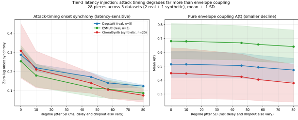
Fig. 4. Corpus-level latency response. Onset synchrony falls much more than the pure envelope channel.
