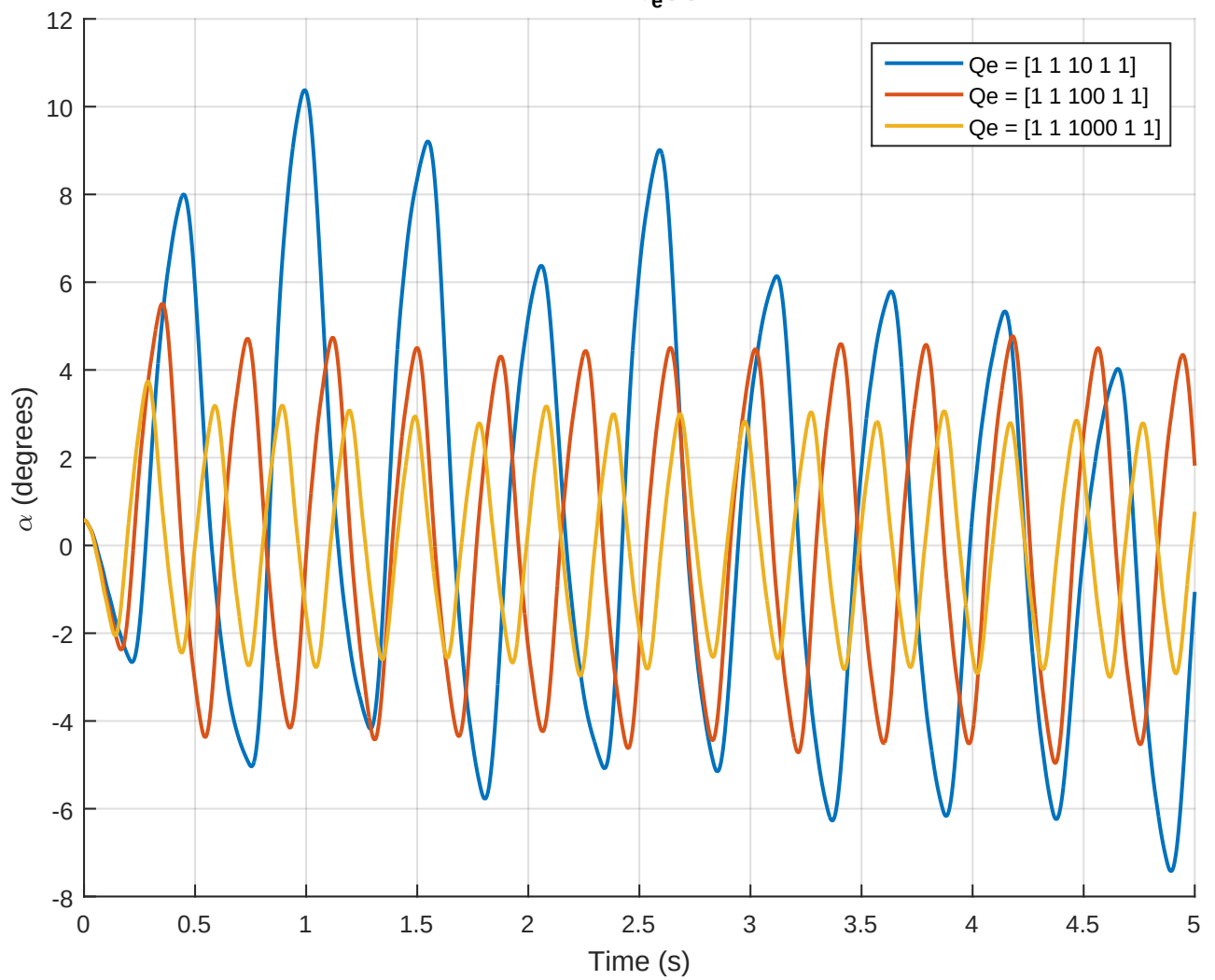
Effect of Q_e(3) on \alpha
