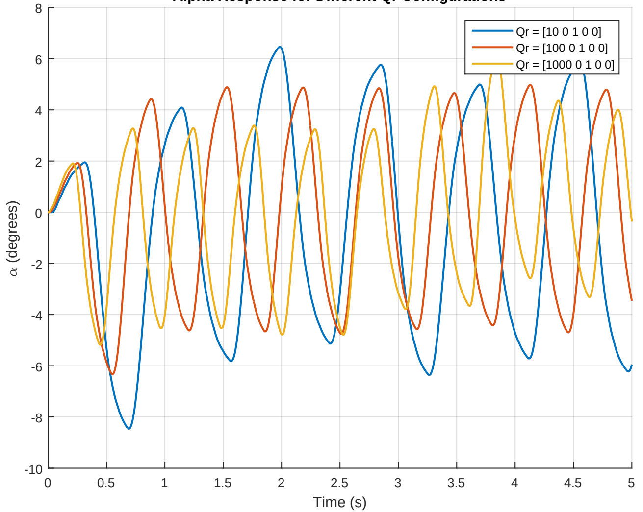
Alpha Response for Different Qr Configurations
