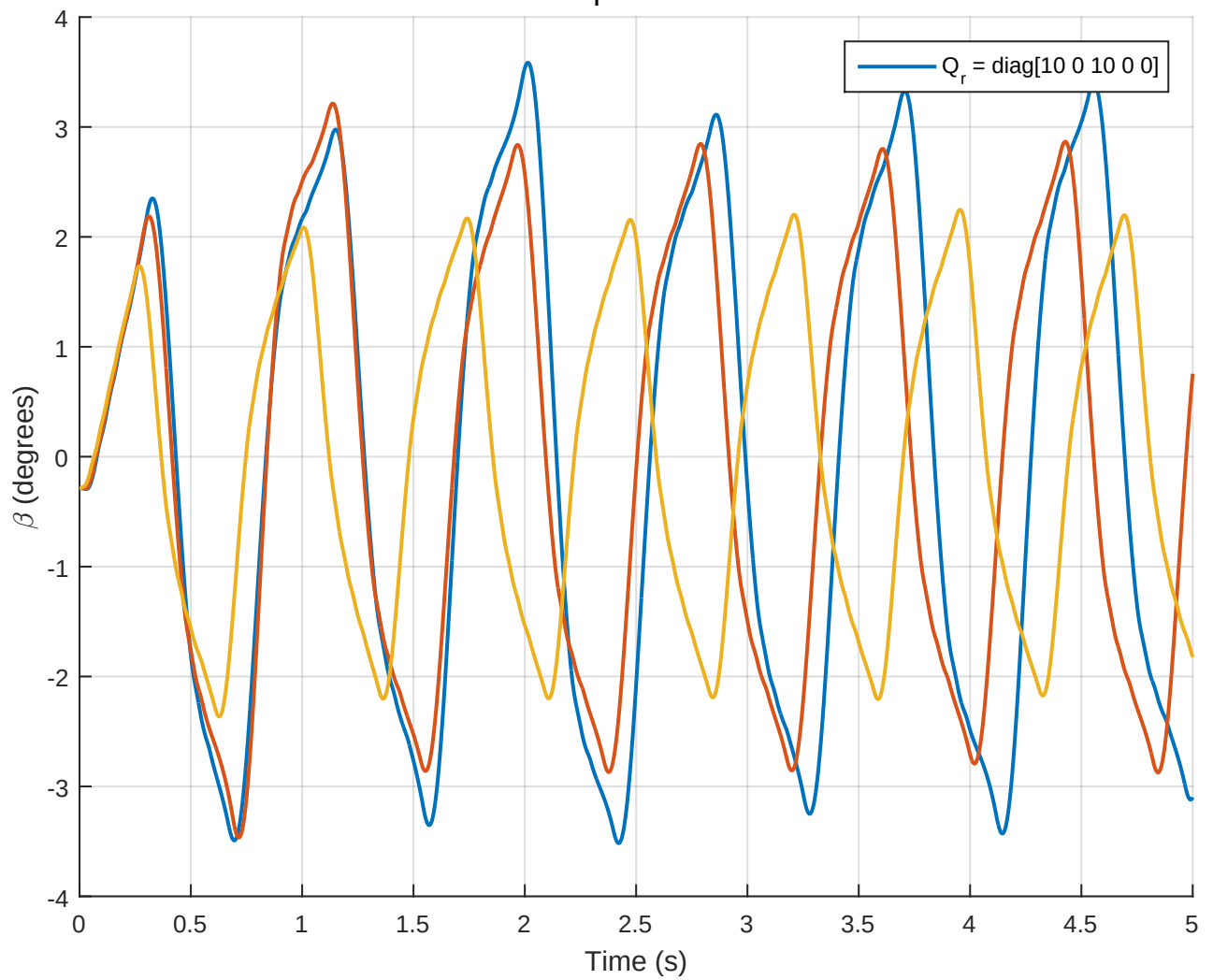
Effect of Q_r on \beta (Tests 4-6)
