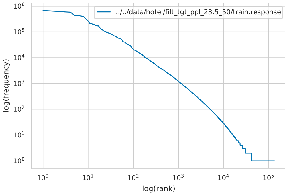
Zipf's law
