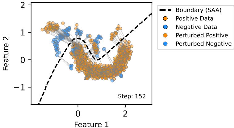
SAA Boundary with WGF Perturbations
