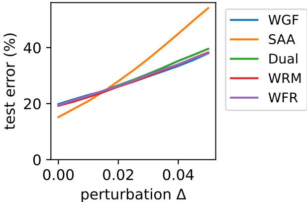
Test error on CIFAR-10 Features
