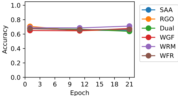
Testing accuracy under PGD Attack
