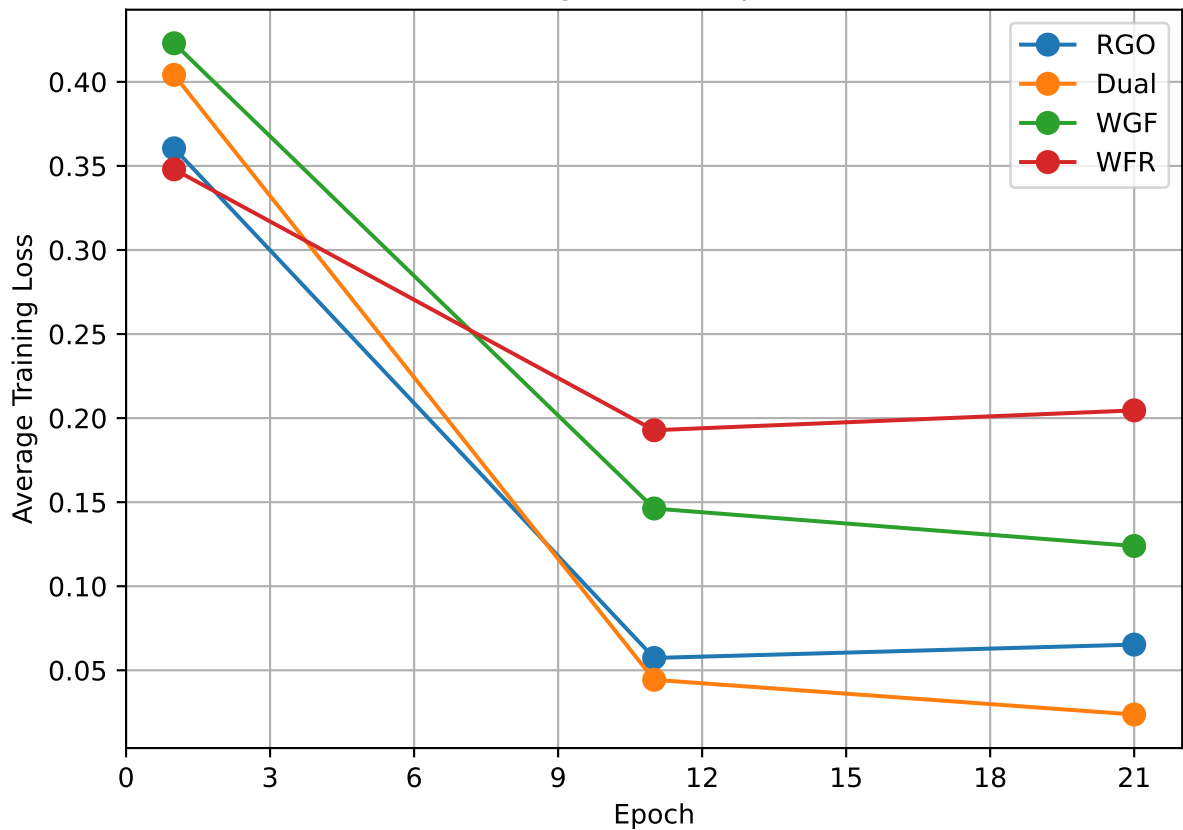
Training Loss Comparison
