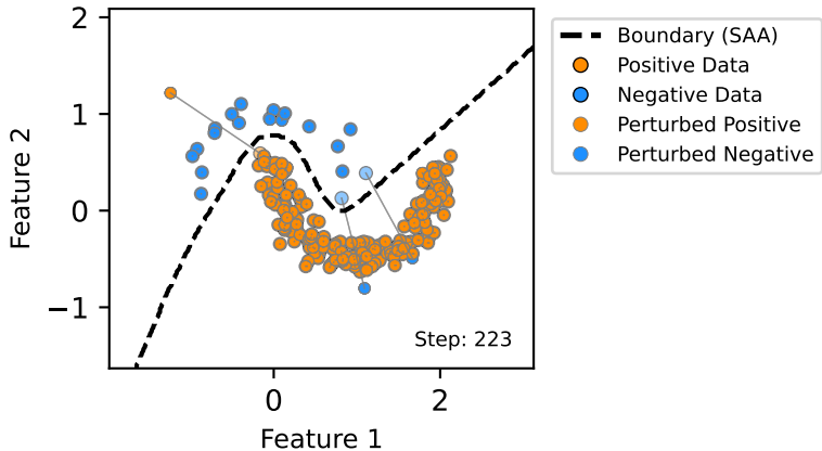
SAA Boundary with WRM Perturbations
